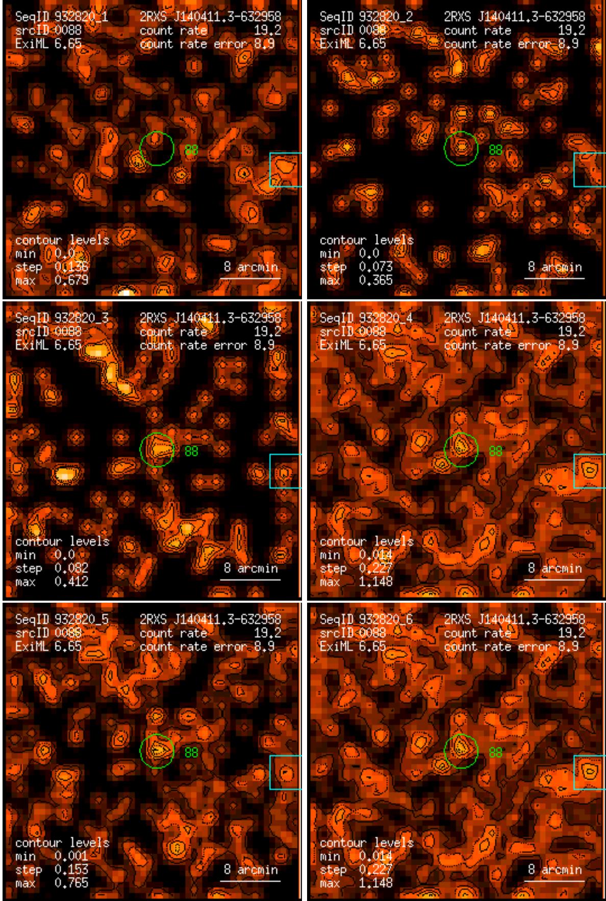
Figure 88: RASS 932820: detection 0088: band rate images, Gaussian filter: (1) PSPC channels 11 – 41, (2) 52 – 90, (3) 91 – 201, (4) 11 – 235, (5) 52 – 201, (6) 11 – 201. Broad band rates in counts/ks. Band rate contour levels in counts/ks/arcmin 2 .
