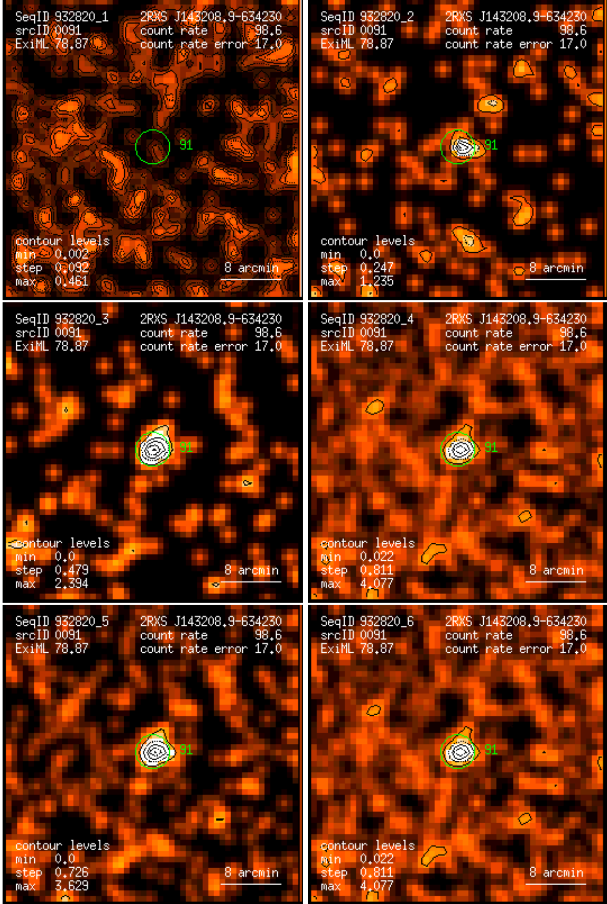
Figure 91: RASS 932820: detection 0091: band rate images, Gaussian filter: (1) PSPC channels 11 – 41, (2) 52 – 90, (3) 91 – 201, (4) 11 – 235, (5) 52 – 201, (6) 11 – 201. Broad band rates in counts/ks. Band rate contour levels in counts/ks/arcmin 2 .
