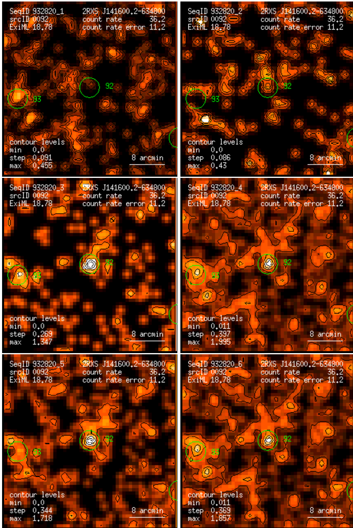
Figure 92: RASS 932820: detection 0092: band rate images, Gaussian filter: (1) PSPC channels 11 – 41, (2) 52 – 90, (3) 91 – 201, (4) 11 – 235, (5) 52 – 201, (6) 11 – 201. Broad band rates in counts/ks. Band rate contour levels in counts/ks/arcmin 2 .
