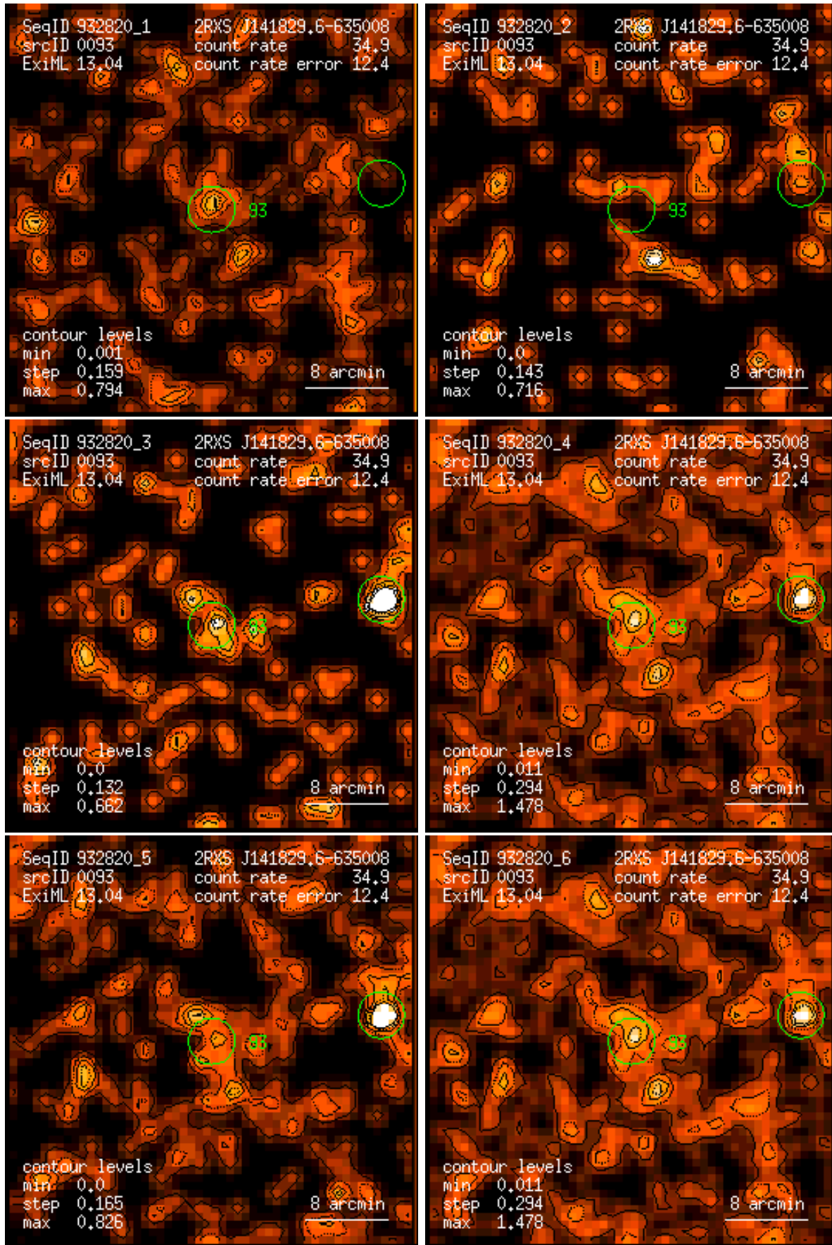
Figure 93: RASS 932820: detection 0093: band rate images, Gaussian filter: (1) PSPC channels 11 – 41, (2) 52 – 90, (3) 91 – 201, (4) 11 – 235, (5) 52 – 201, (6) 11 – 201. Broad band rates in counts/ks. Band rate contour levels in counts/ks/arcmin 2 .
