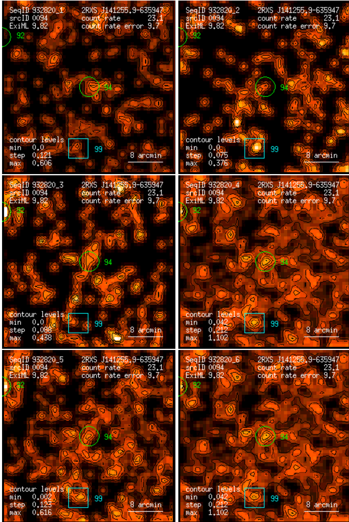
Figure 94: RASS 932820: detection 0094: band rate images, Gaussian filter: (1) PSPC channels 11 – 41, (2) 52 – 90, (3) 91 – 201, (4) 11 – 235, (5) 52 – 201, (6) 11 – 201. Broad band rates in counts/ks. Band rate contour levels in counts/ks/arcmin 2 .
