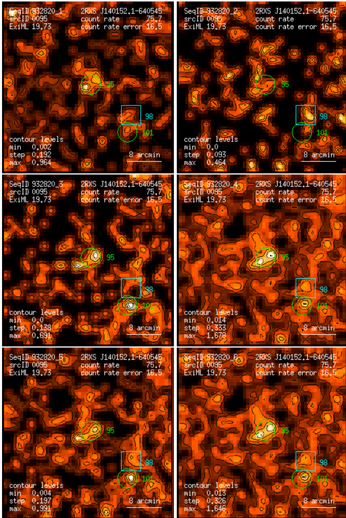
Figure 95: RASS 932820: detection 0095: band rate images, Gaussian filter: (1) PSPC channels 11 – 41, (2) 52 – 90, (3) 91 – 201, (4) 11 – 235, (5) 52 – 201, (6) 11 – 201. Broad band rates in counts/ks. Band rate contour levels in counts/ks/arcmin 2 .
