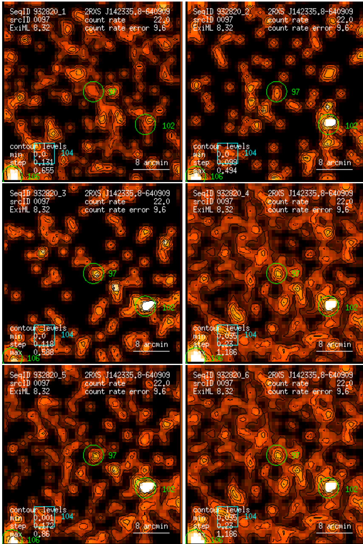
Figure 97: RASS 932820: detection 0097: band rate images, Gaussian filter: (1) PSPC channels 11 – 41, (2) 52 – 90, (3) 91 – 201, (4) 11 – 235, (5) 52 – 201, (6) 11 – 201. Broad band rates in counts/ks. Band rate contour levels in counts/ks/arcmin 2 .
