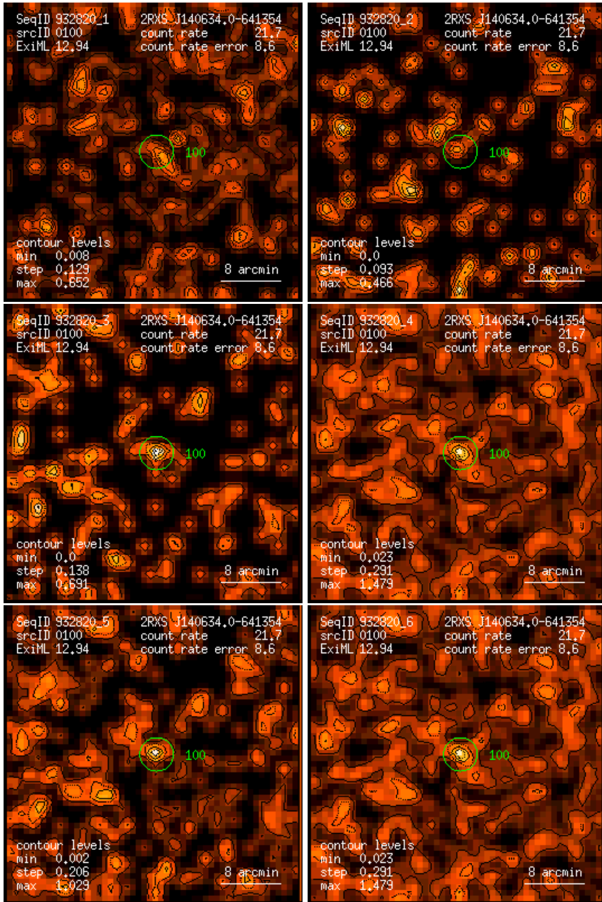
Figure 100: RASS 932820: detection 0100: band rate images, Gaussian filter: (1) PSPC channels 11 – 41, (2) 52 – 90, (3) 91 – 201, (4) 11 – 235, (5) 52 – 201, (6) 11 – 201. Broad band rates in counts/ks. Band rate contour levels in counts/ks/arcmin 2 .
