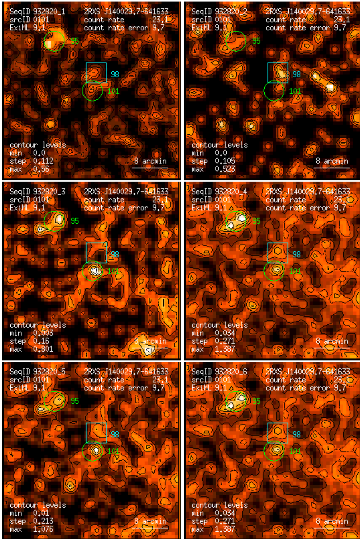
Figure 101: RASS 932820: detection 0101: band rate images, Gaussian filter: (1) PSPC channels 11 – 41, (2) 52 – 90, (3) 91 – 201, (4) 11 – 235, (5) 52 – 201, (6) 11 – 201. Broad band rates in counts/ks. Band rate contour levels in counts/ks/arcmin 2 .
