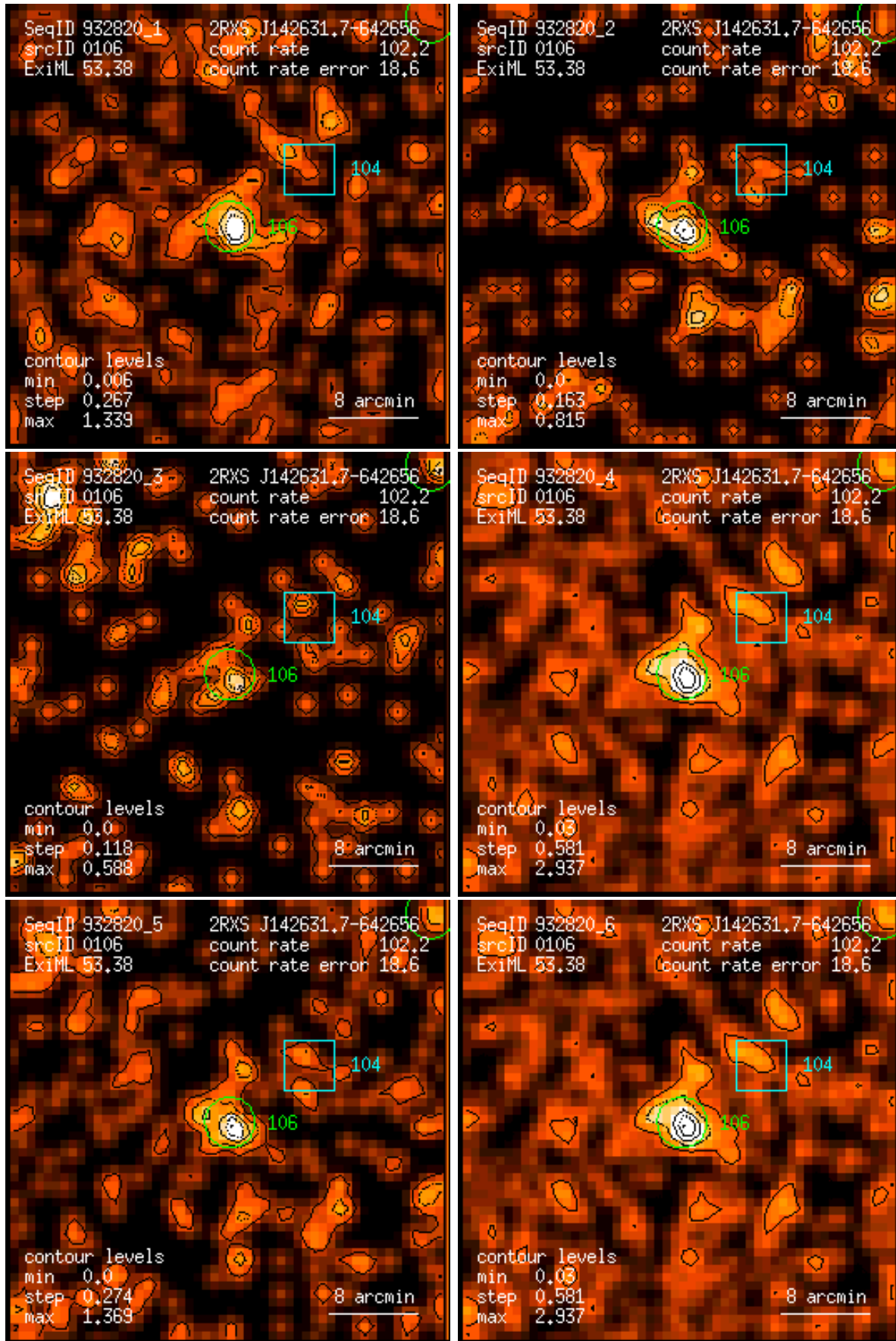
Figure 106: RASS 932820: detection 0106: band rate images, Gaussian filter: (1) PSPC channels 11 – 41, (2) 52 – 90, (3) 91 – 201, (4) 11 – 235, (5) 52 – 201, (6) 11 – 201. Broad band rates in counts/ks. Band rate contour levels in counts/ks/arcmin 2 .
