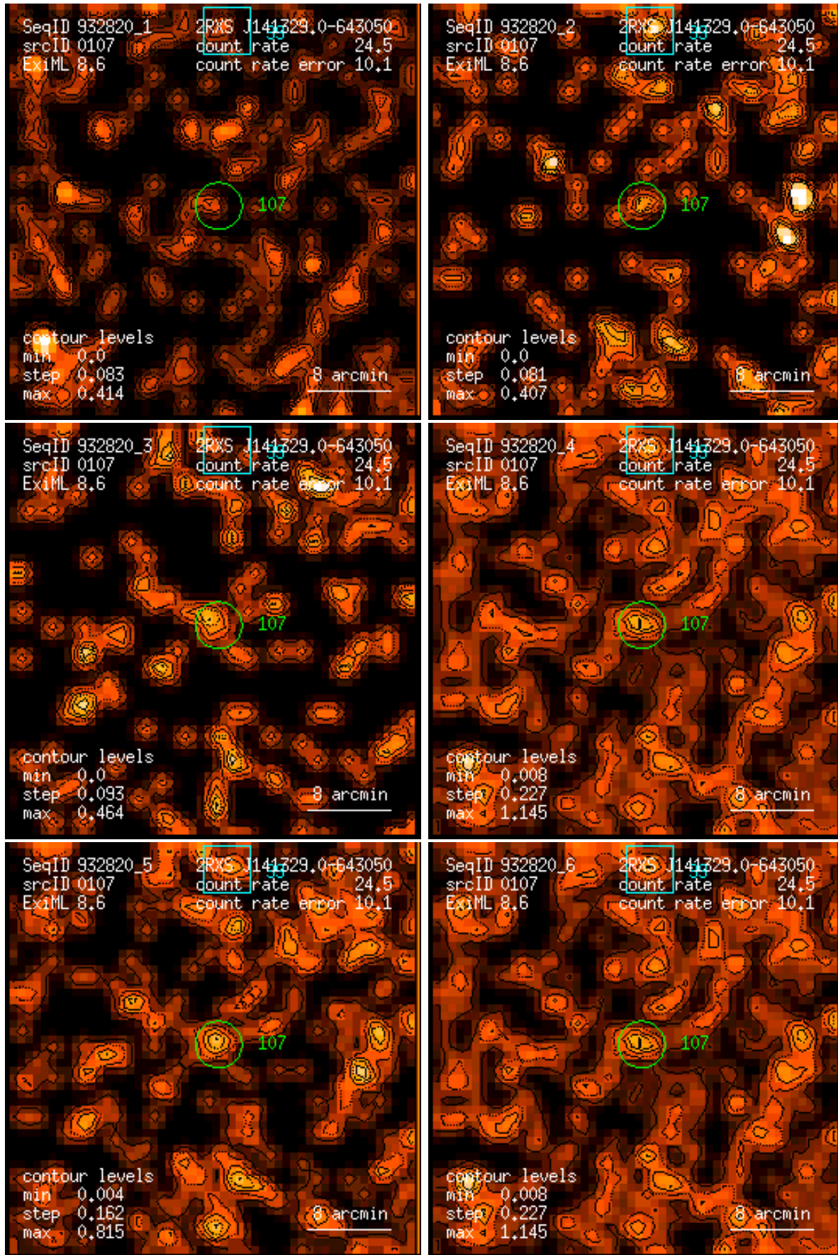
Figure 107: RASS 932820: detection 0107: band rate images, Gaussian filter: (1) PSPC channels 11 – 41, (2) 52 – 90, (3) 91 – 201, (4) 11 – 235, (5) 52 – 201, (6) 11 – 201. Broad band rates in counts/ks. Band rate contour levels in counts/ks/arcmin 2 .
