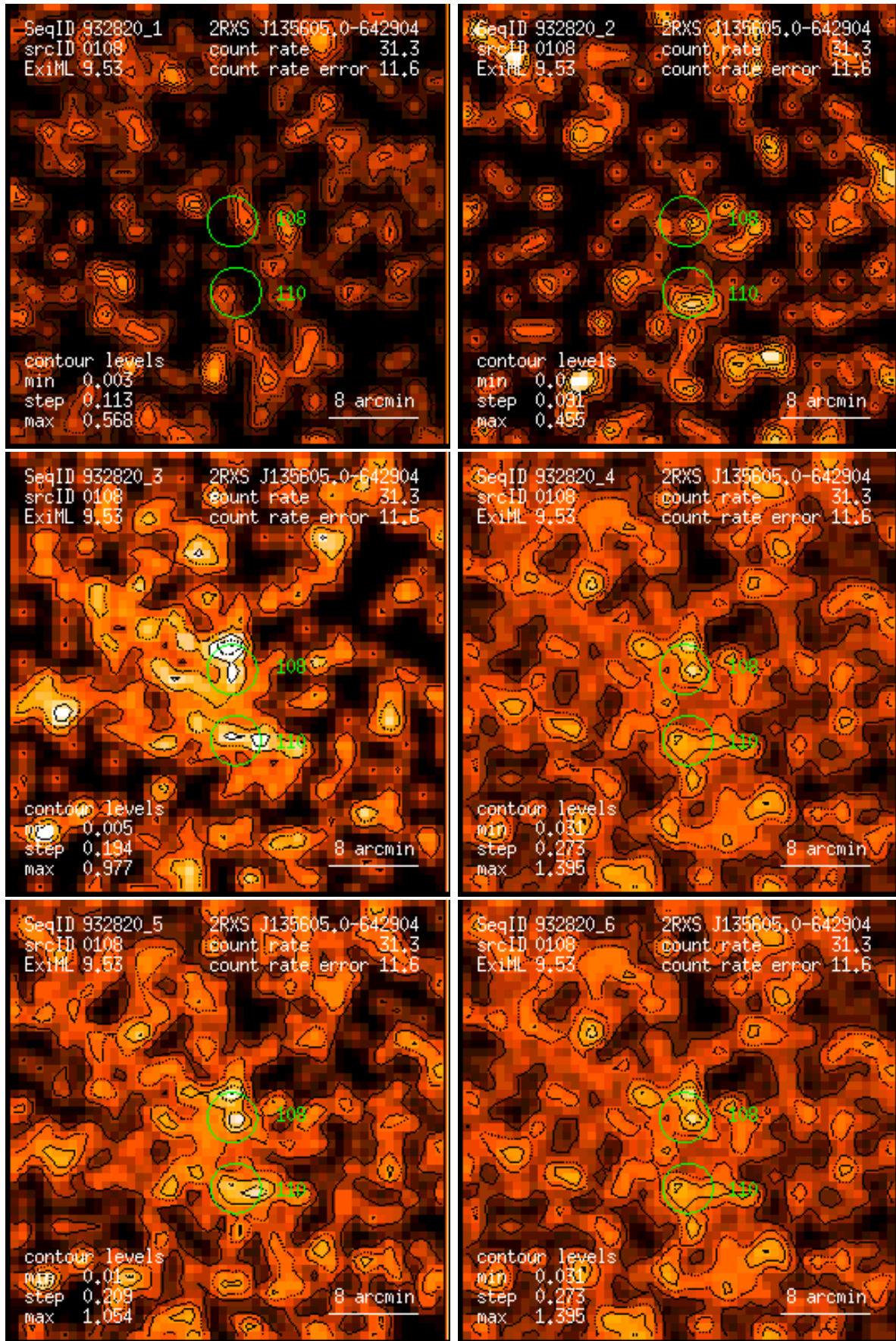
Figure 108: RASS 932820: detection 0108: band rate images, Gaussian filter: (1) PSPC channels 11 – 41, (2) 52 – 90, (3) 91 – 201, (4) 11 – 235, (5) 52 – 201, (6) 11 – 201. Broad band rates in counts/ks. Band rate contour levels in counts/ks/arcmin 2 .
