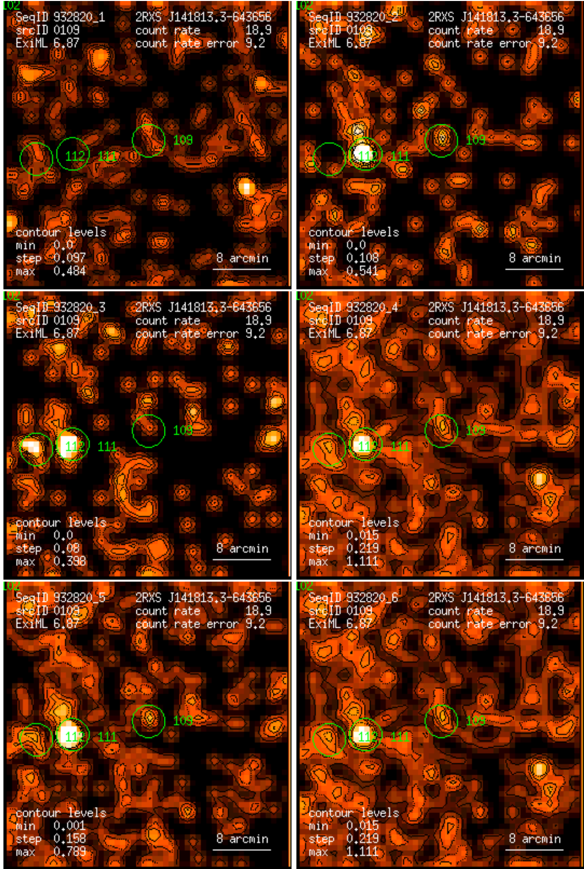
Figure 109: RASS 932820: detection 0109: band rate images, Gaussian filter: (1) PSPC channels 11 – 41, (2) 52 – 90, (3) 91 – 201, (4) 11 – 235, (5) 52 – 201, (6) 11 – 201. Broad band rates in counts/ks. Band rate contour levels in counts/ks/arcmin 2 .
