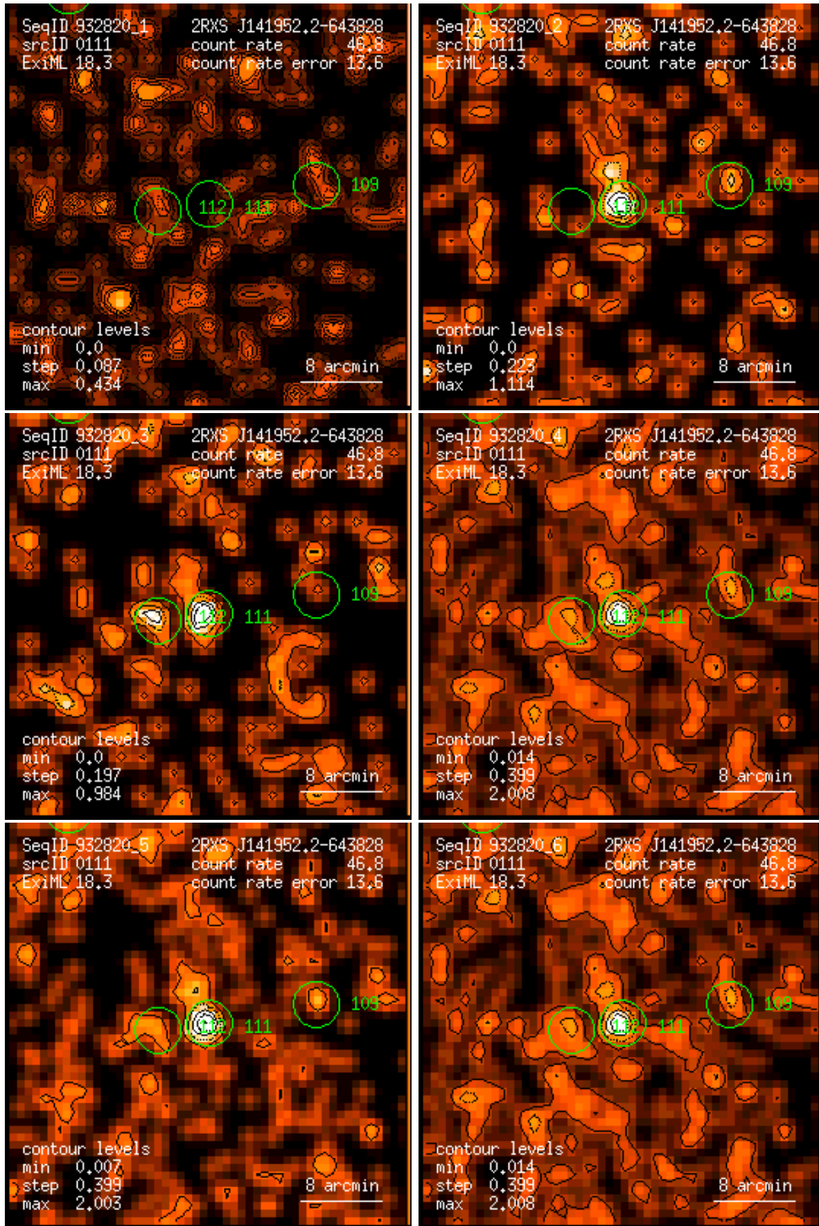
Figure 111: RASS 932820: detection 0111: band rate images, Gaussian filter: (1) PSPC channels 11 – 41, (2) 52 – 90, (3) 91 – 201, (4) 11 – 235, (5) 52 – 201, (6) 11 – 201. Broad band rates in counts/ks. Band rate contour levels in counts/ks/arcmin 2 .
