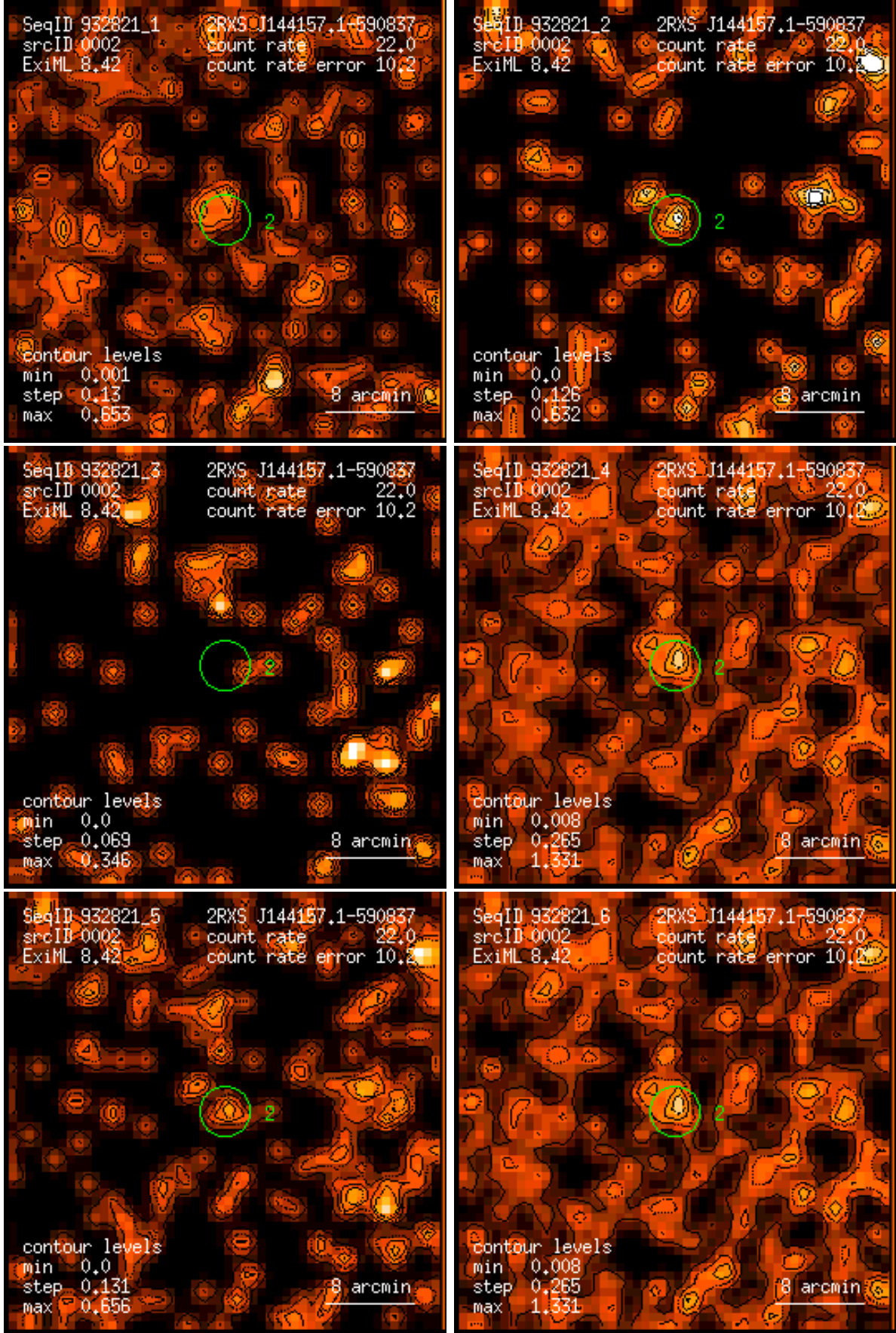
Figure 2: RASS 932821: detection 0002: band rate images, Gaussian filter: (1) PSPC channels 11 – 41, (2) 52 – 90, (3) 91 – 201, (4) 11 – 235, (5) 52 – 201, (6) 11 – 201. Broad band rates in counts/ks. Band rate contour levels in counts/ks/arcmin 2 .
