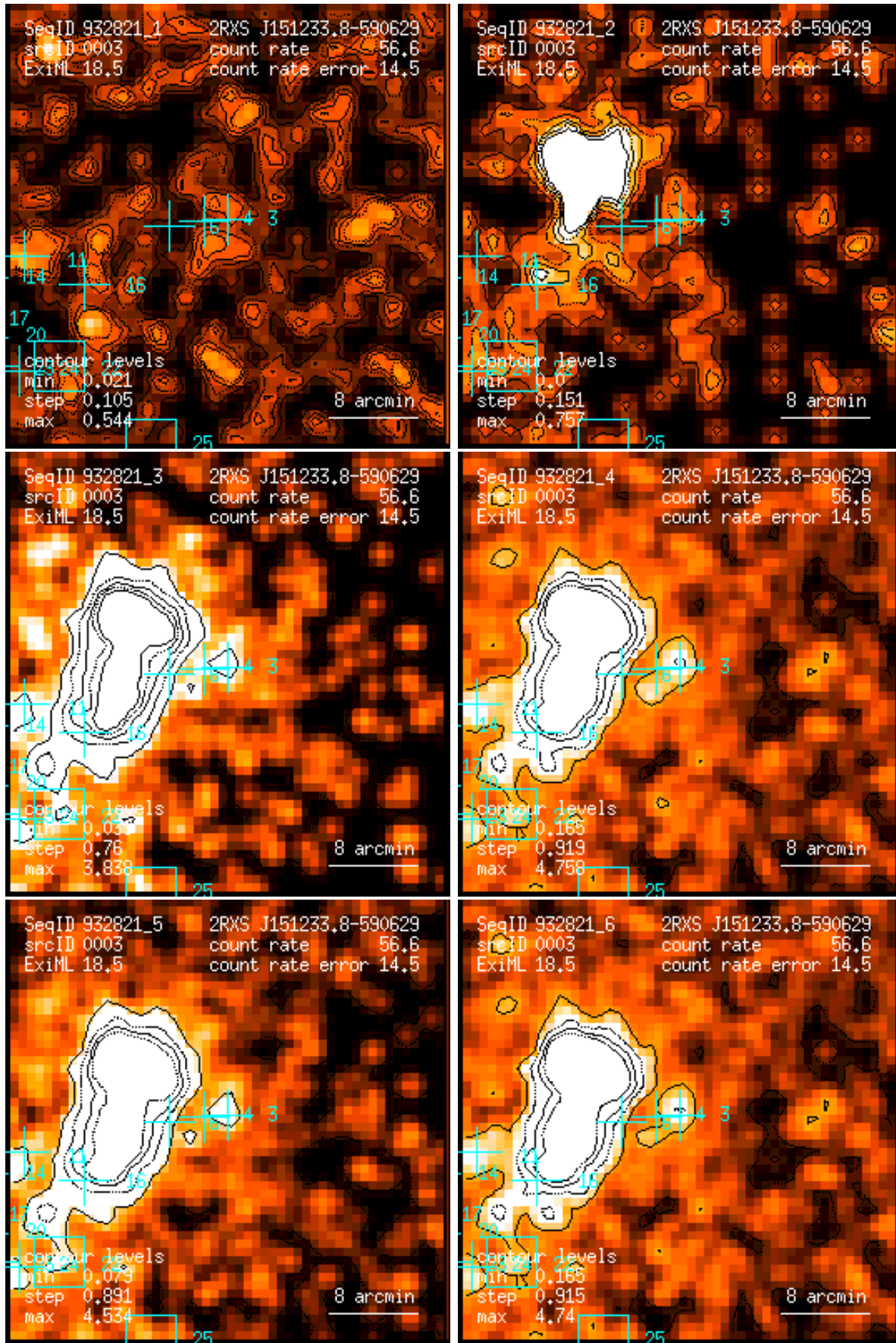
Figure 3: RASS 932821: detection 0003: band rate images, Gaussian filter: (1) PSPC channels 11 – 41, (2) 52 – 90, (3) 91 – 201, (4) 11 – 235, (5) 52 – 201, (6) 11 – 201. Broad band rates in counts/ks. Band rate contour levels in counts/ks/arcmin 2 .
