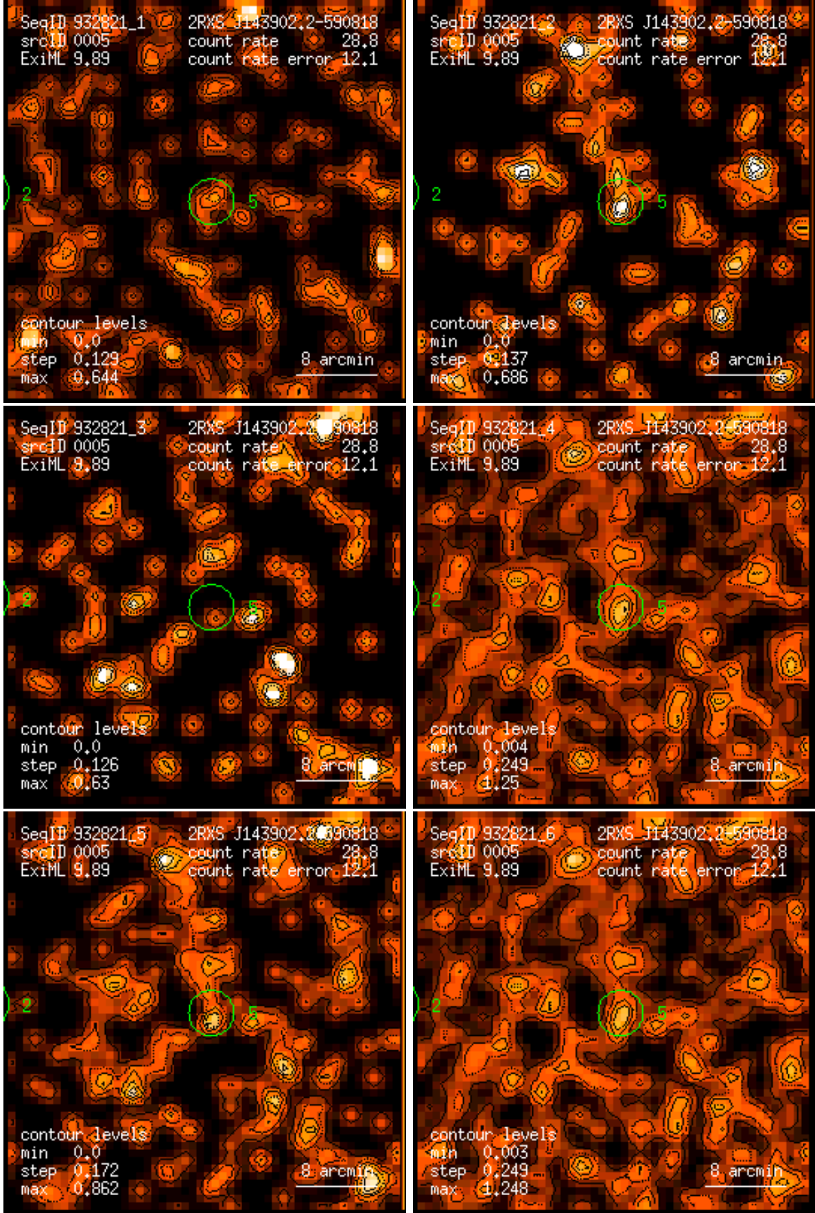
Figure 5: RASS 932821: detection 0005: band rate images, Gaussian filter: (1) PSPC channels 11 – 41, (2) 52 – 90, (3) 91 – 201, (4) 11 – 235, (5) 52 – 201, (6) 11 – 201. Broad band rates in counts/ks. Band rate contour levels in counts/ks/arcmin 2 .
