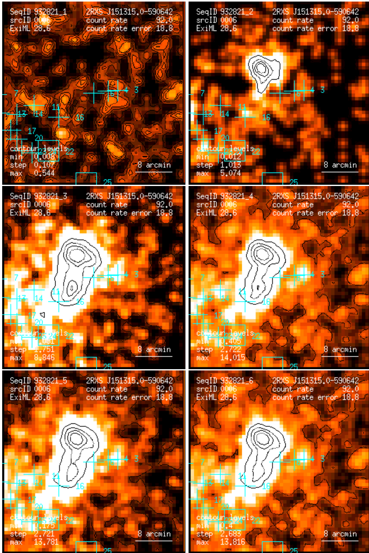
Figure 6: RASS 932821: detection 0006: band rate images, Gaussian filter: (1) PSPC channels 11 – 41, (2) 52 – 90, (3) 91 – 201, (4) 11 – 235, (5) 52 – 201, (6) 11 – 201. Broad band rates in counts/ks. Band rate contour levels in counts/ks/arcmin 2 .
