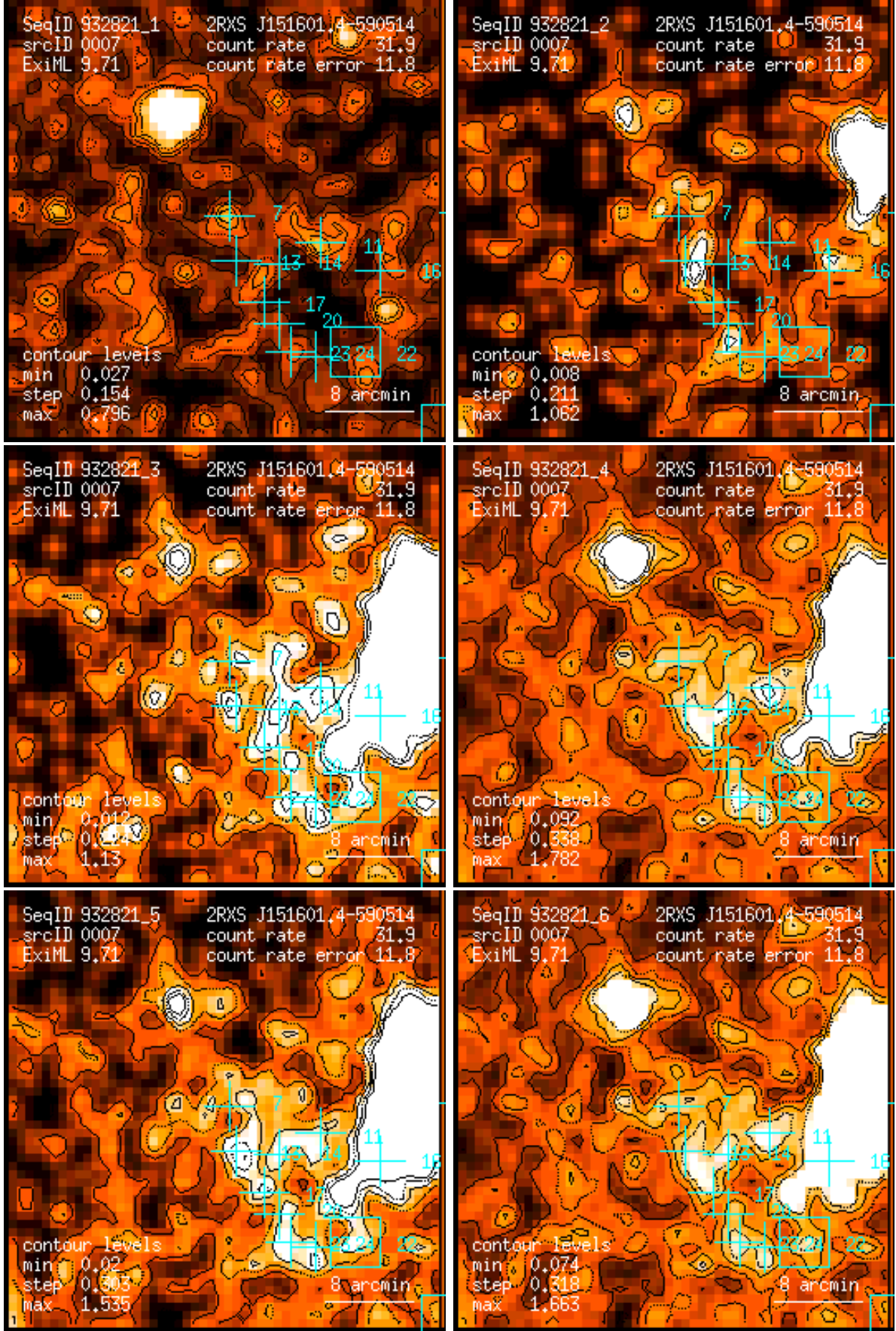
Figure 7: RASS 932821: detection 0007: band rate images, Gaussian filter: (1) PSPC channels 11 – 41, (2) 52 – 90, (3) 91 – 201, (4) 11 – 235, (5) 52 – 201, (6) 11 – 201. Broad band rates in counts/ks. Band rate contour levels in counts/ks/arcmin 2 .
