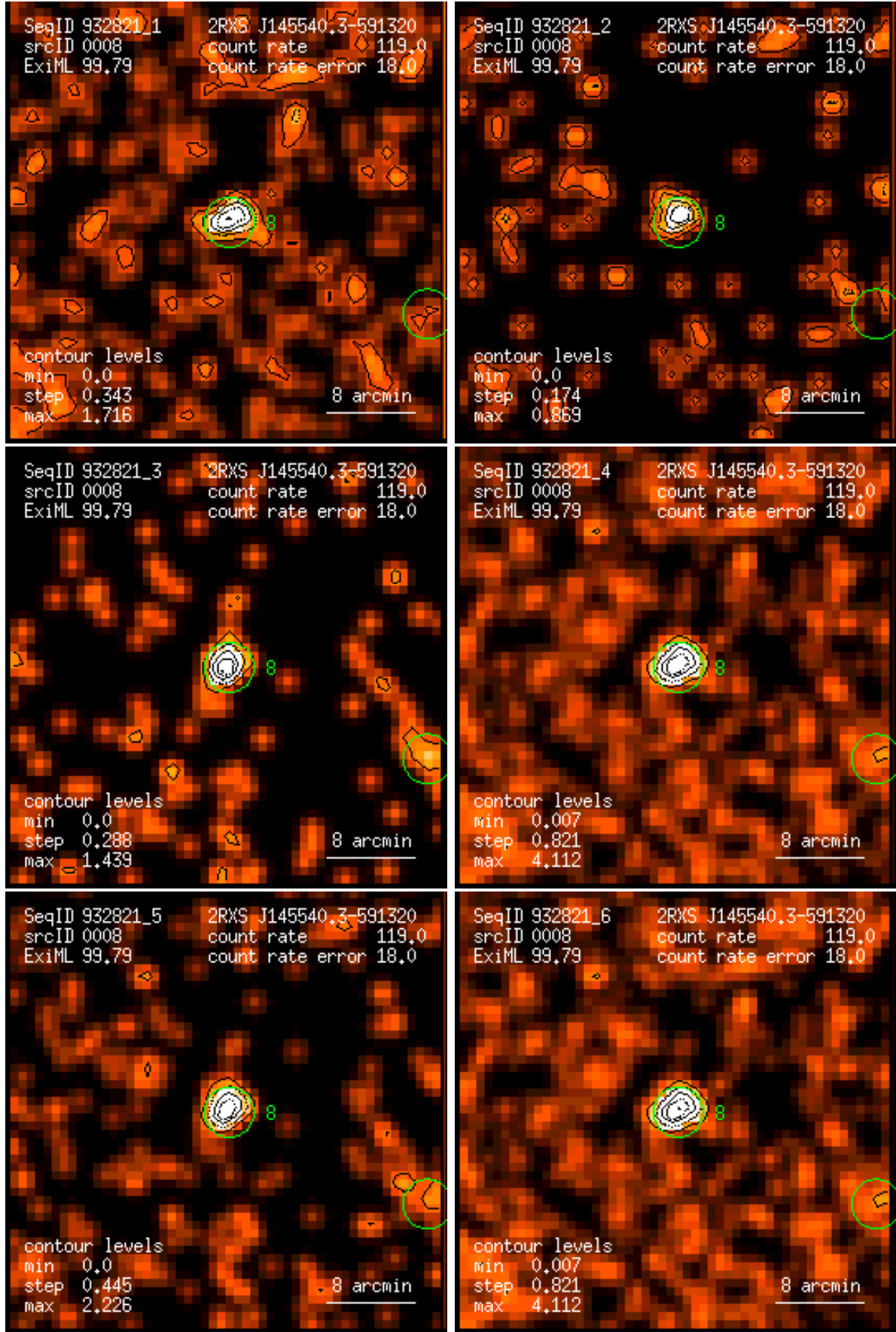
Figure 8: RASS 932821: detection 0008: band rate images, Gaussian filter: (1) PSPC channels 11 – 41, (2) 52 – 90, (3) 91 – 201, (4) 11 – 235, (5) 52 – 201, (6) 11 – 201. Broad band rates in counts/ks. Band rate contour levels in counts/ks/arcmin 2 .
