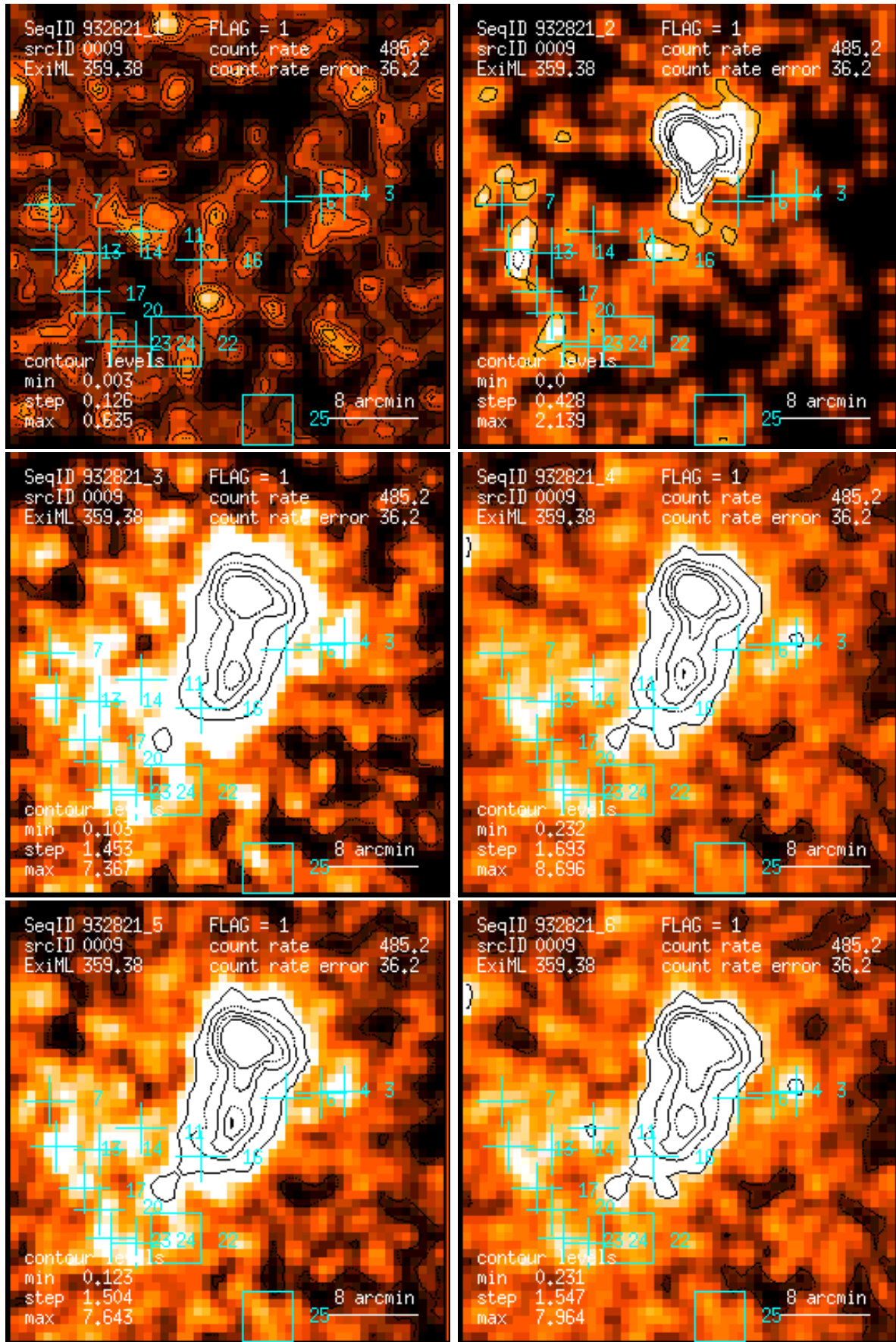
Figure 9: RASS 932821: detection 0009: band rate images, Gaussian filter: (1) PSPC channels 11 – 41, (2) 52 – 90, (3) 91 – 201, (4) 11 – 235, (5) 52 – 201, (6) 11 – 201. Broad band rates in counts/ks. Band rate contour levels in counts/ks/arcmin 2 .
