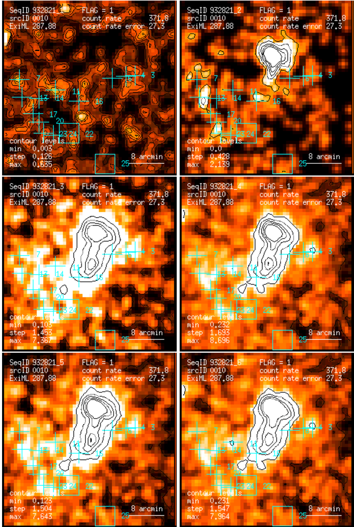
Figure 10: RASS 932821: detection 0010: band rate images, Gaussian filter: (1) PSPC channels 11 – 41, (2) 52 – 90, (3) 91 – 201, (4) 11 – 235, (5) 52 – 201, (6) 11 – 201. Broad band rates in counts/ks. Band rate contour levels in counts/ks/arcmin 2 .
