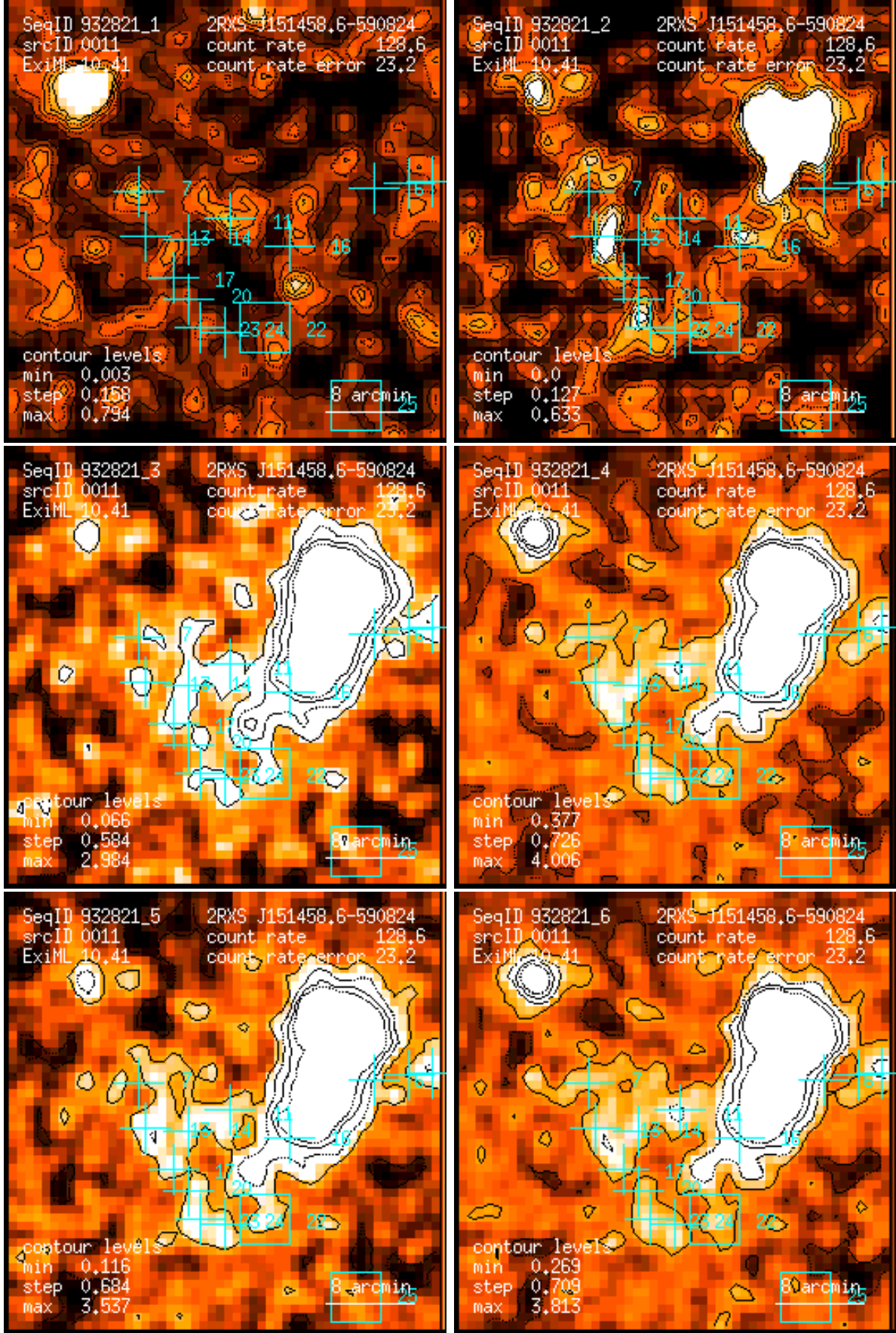
Figure 11: RASS 932821: detection 0011: band rate images, Gaussian filter: (1) PSPC channels 11 – 41, (2) 52 – 90, (3) 91 – 201, (4) 11 – 235, (5) 52 – 201, (6) 11 – 201. Broad band rates in counts/ks. Band rate contour levels in counts/ks/arcmin 2 .
