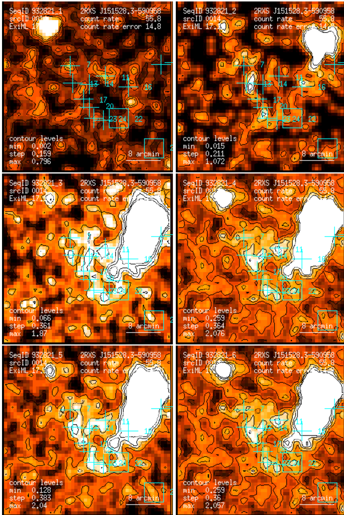
Figure 14: RASS 932821: detection 0014: band rate images, Gaussian filter: (1) PSPC channels 11 – 41, (2) 52 – 90, (3) 91 – 201, (4) 11 – 235, (5) 52 – 201, (6) 11 – 201. Broad band rates in counts/ks. Band rate contour levels in counts/ks/arcmin 2 .
