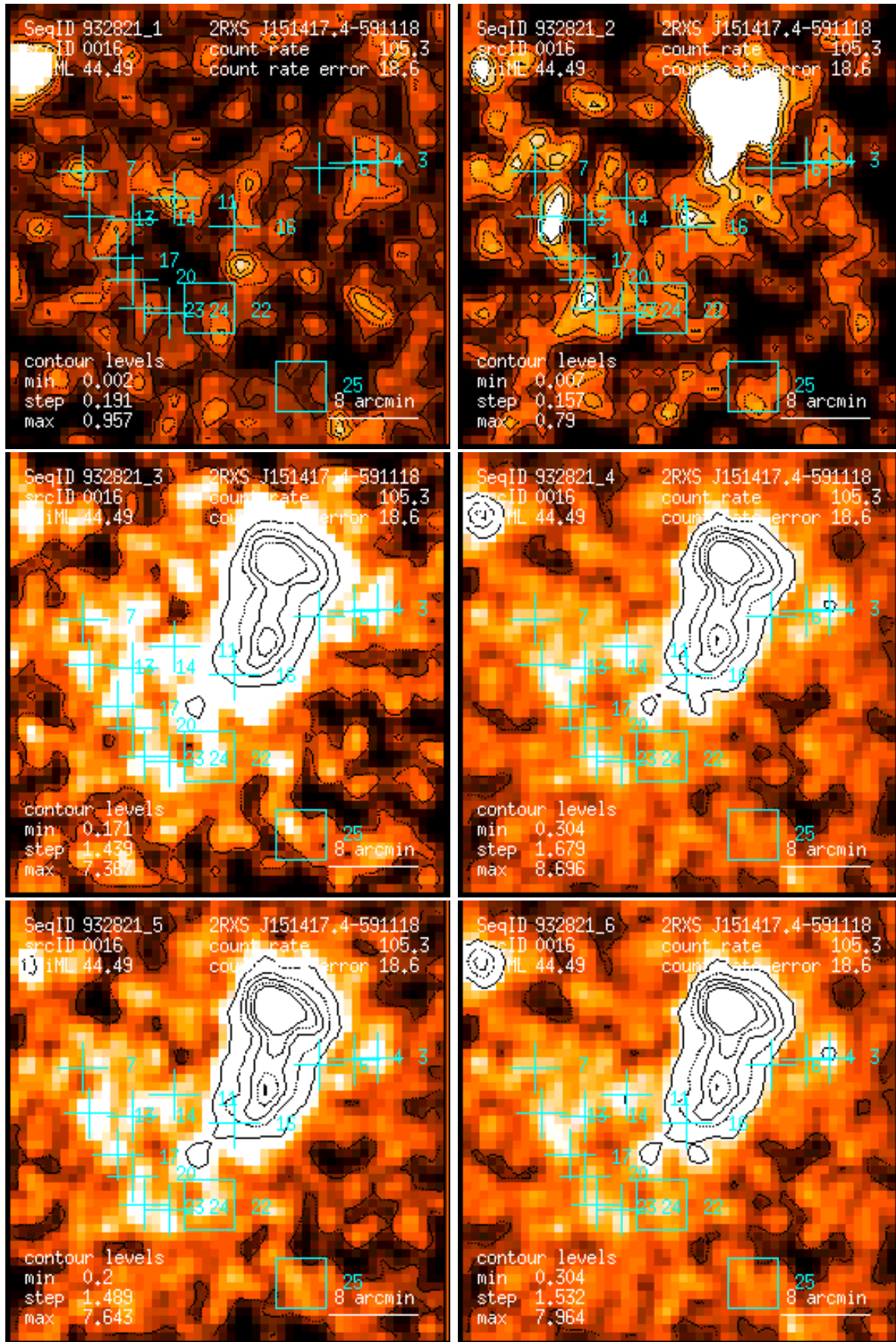
Figure 16: RASS 932821: detection 0016: band rate images, Gaussian filter: (1) PSPC channels 11 – 41, (2) 52 – 90, (3) 91 – 201, (4) 11 – 235, (5) 52 – 201, (6) 11 – 201. Broad band rates in counts/ks. Band rate contour levels in counts/ks/arcmin 2 .
