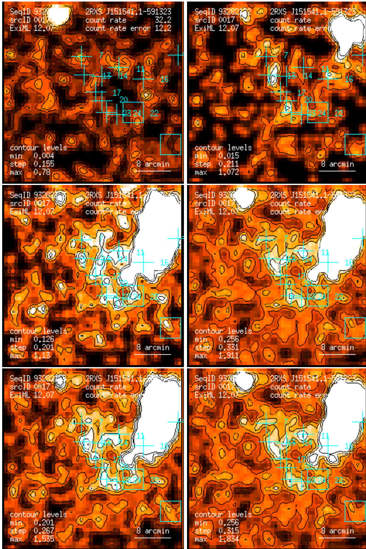
Figure 17: RASS 932821: detection 0017: band rate images, Gaussian filter: (1) PSPC channels 11 – 41, (2) 52 – 90, (3) 91 – 201, (4) 11 – 235, (5) 52 – 201, (6) 11 – 201. Broad band rates in counts/ks. Band rate contour levels in counts/ks/arcmin 2 .
