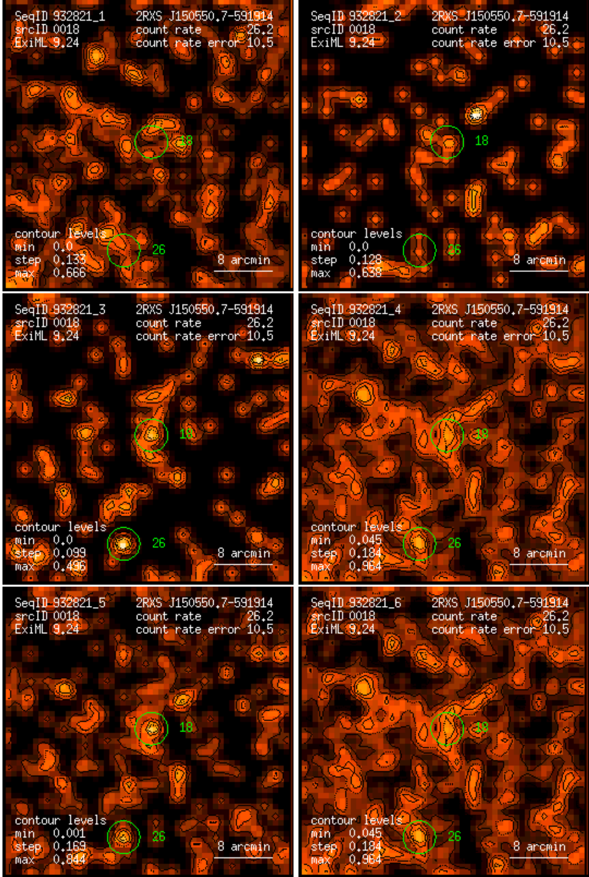
Figure 18: RASS 932821: detection 0018: band rate images, Gaussian filter: (1) PSPC channels 11 – 41, (2) 52 – 90, (3) 91 – 201, (4) 11 – 235, (5) 52 – 201, (6) 11 – 201. Broad band rates in counts/ks. Band rate contour levels in counts/ks/arcmin 2 .
