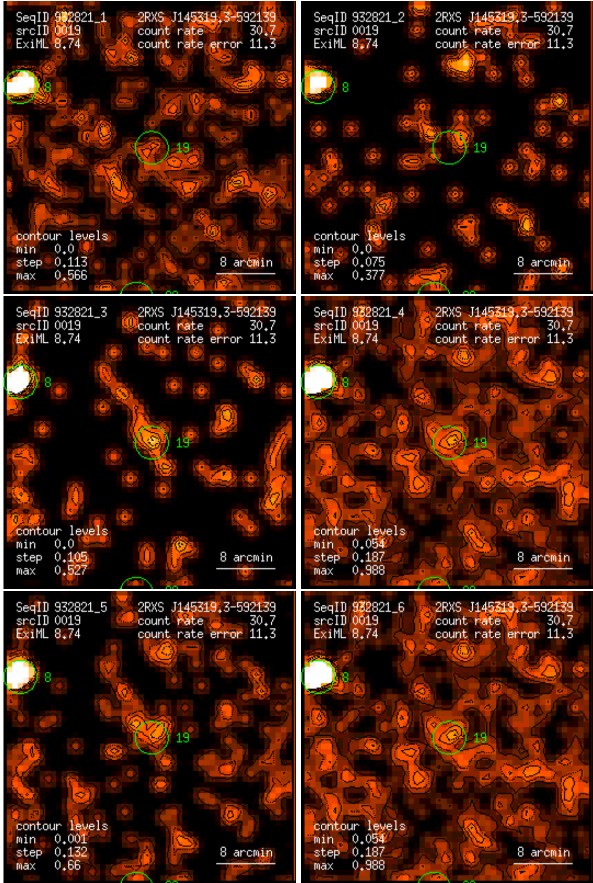
Figure 19: RASS 932821: detection 0019: band rate images, Gaussian filter: (1) PSPC channels 11 – 41, (2) 52 – 90, (3) 91 – 201, (4) 11 – 235, (5) 52 – 201, (6) 11 – 201. Broad band rates in counts/ks. Band rate contour levels in counts/ks/arcmin 2 .
