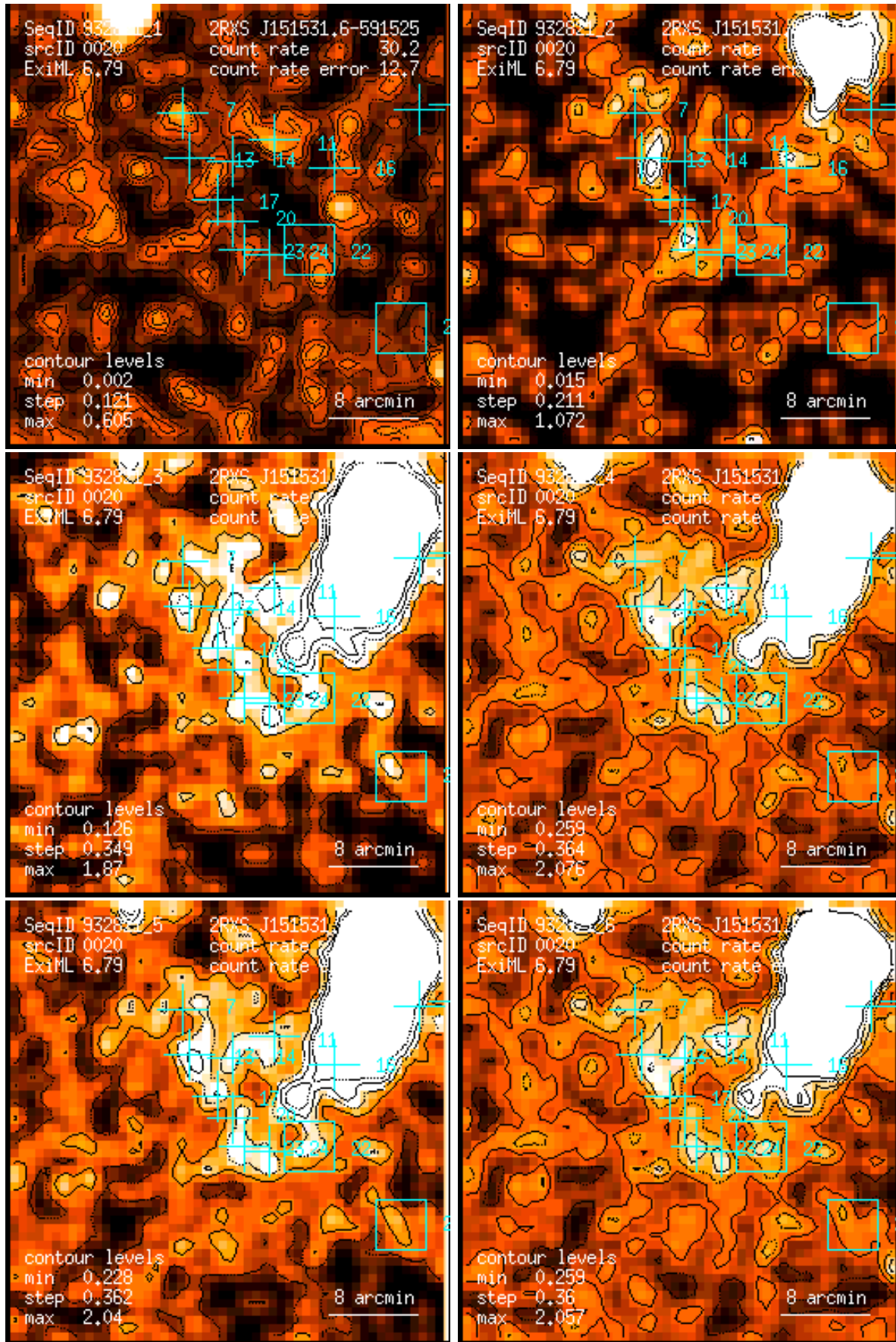
Figure 20: RASS 932821: detection 0020: band rate images, Gaussian filter: (1) PSPC channels 11 – 41, (2) 52 – 90, (3) 91 – 201, (4) 11 – 235, (5) 52 – 201, (6) 11 – 201. Broad band rates in counts/ks. Band rate contour levels in counts/ks/arcmin 2 .
