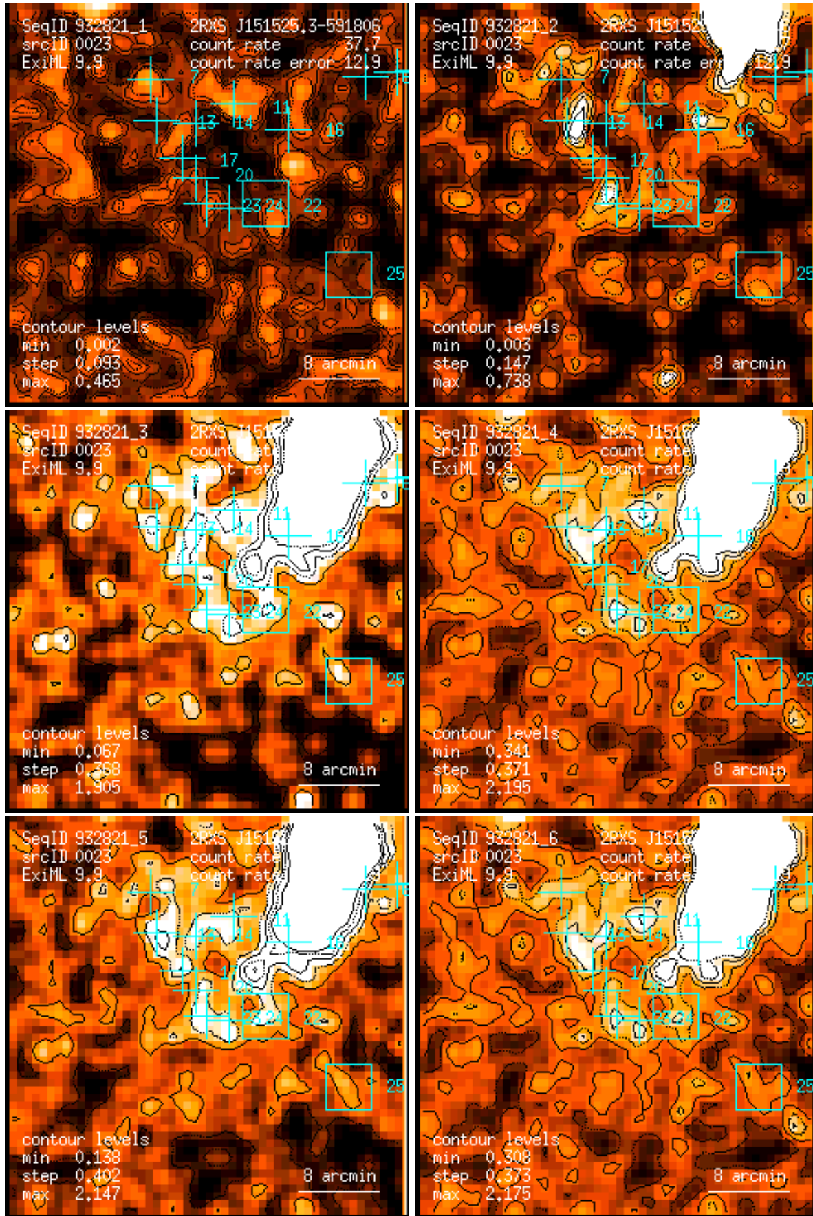
Figure 23: RASS 932821: detection 0023: band rate images, Gaussian filter: (1) PSPC channels 11 – 41, (2) 52 – 90, (3) 91 – 201, (4) 11 – 235, (5) 52 – 201, (6) 11 – 201. Broad band rates in counts/ks. Band rate contour levels in counts/ks/arcmin 2 .
