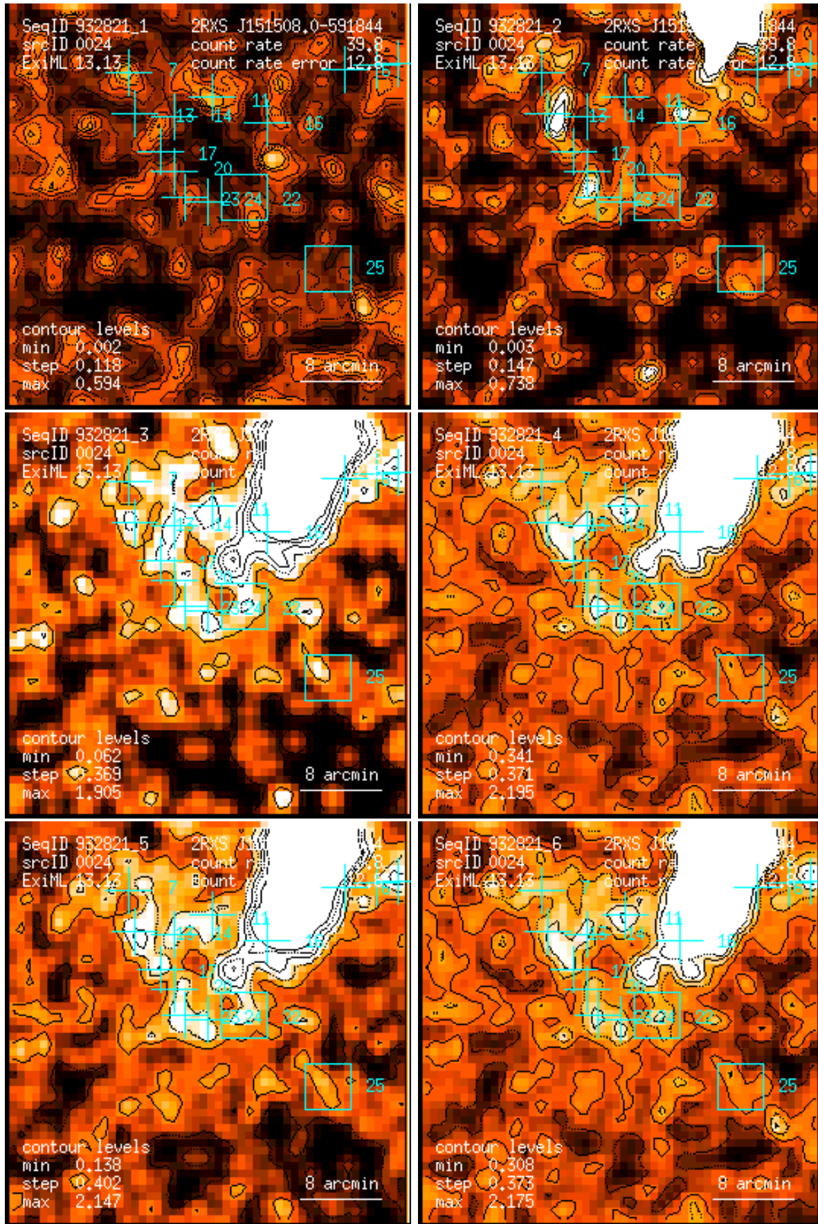
Figure 24: RASS 932821: detection 0024: band rate images, Gaussian filter: (1) PSPC channels 11 – 41, (2) 52 – 90, (3) 91 – 201, (4) 11 – 235, (5) 52 – 201, (6) 11 – 201. Broad band rates in counts/ks. Band rate contour levels in counts/ks/arcmin 2 .
