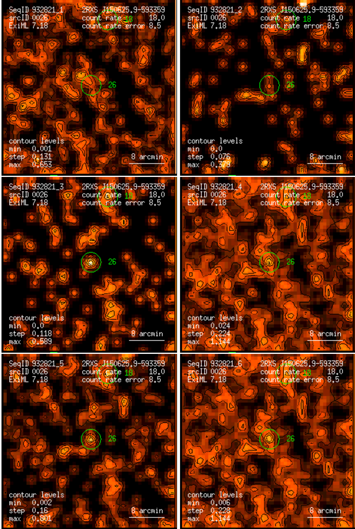
Figure 26: RASS 932821: detection 0026: band rate images, Gaussian filter: (1) PSPC channels 11 – 41, (2) 52 – 90, (3) 91 – 201, (4) 11 – 235, (5) 52 – 201, (6) 11 – 201. Broad band rates in counts/ks. Band rate contour levels in counts/ks/arcmin 2 .
