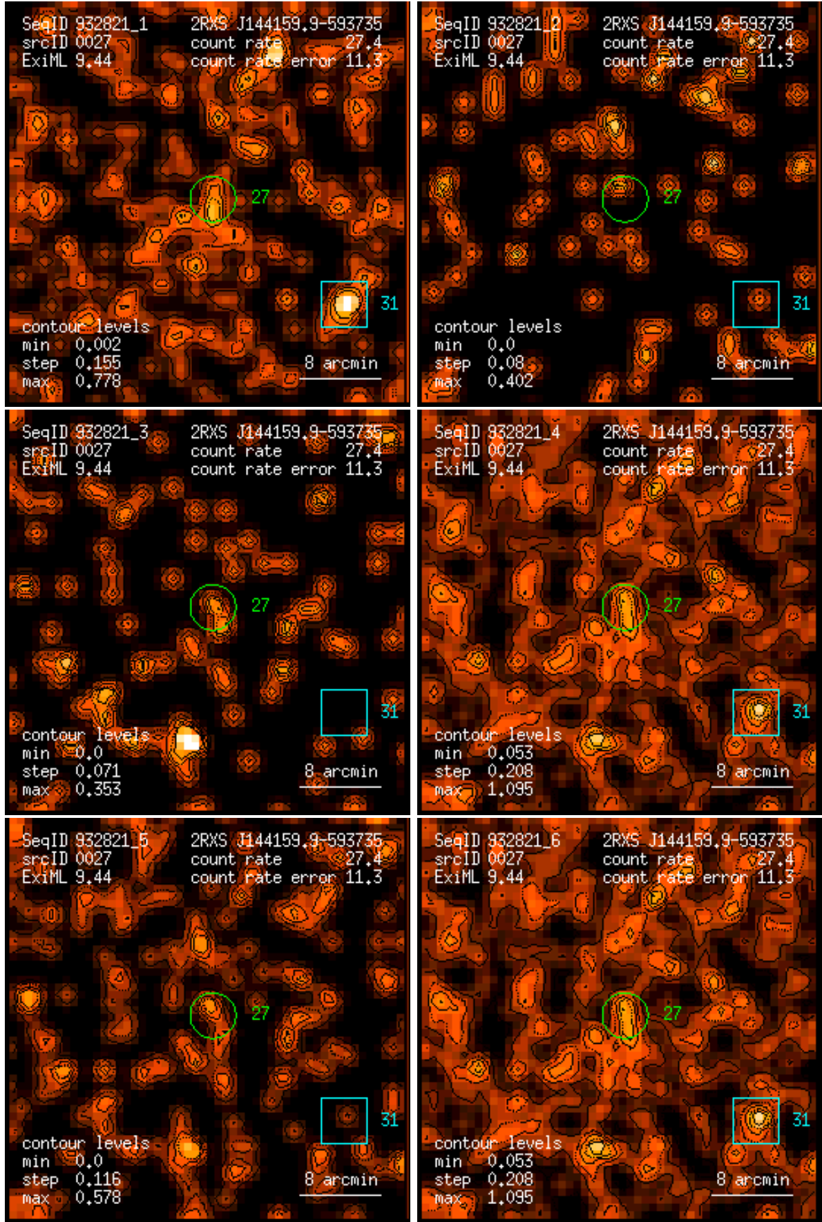
Figure 27: RASS 932821: detection 0027: band rate images, Gaussian filter: (1) PSPC channels 11 – 41, (2) 52 – 90, (3) 91 – 201, (4) 11 – 235, (5) 52 – 201, (6) 11 – 201. Broad band rates in counts/ks. Band rate contour levels in counts/ks/arcmin 2 .
