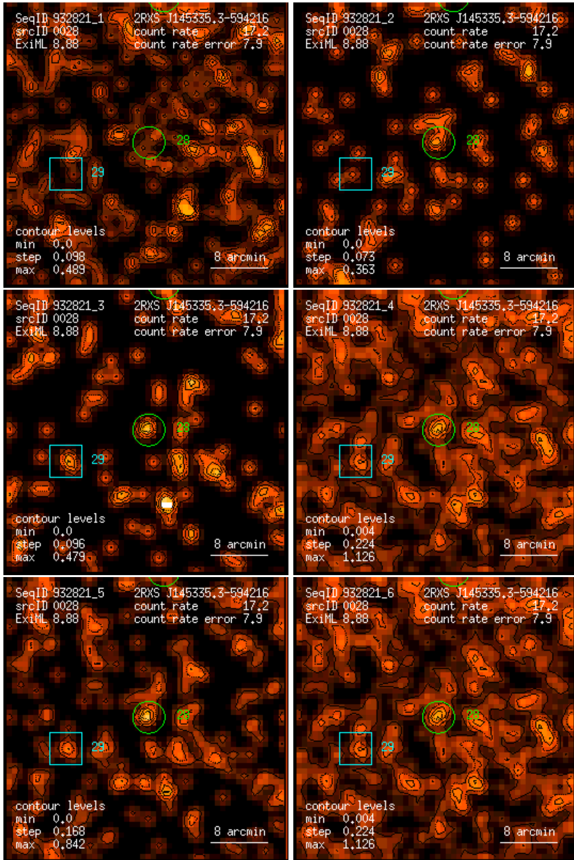
Figure 28: RASS 932821: detection 0028: band rate images, Gaussian filter: (1) PSPC channels 11 – 41, (2) 52 – 90, (3) 91 – 201, (4) 11 – 235, (5) 52 – 201, (6) 11 – 201. Broad band rates in counts/ks. Band rate contour levels in counts/ks/arcmin 2 .
