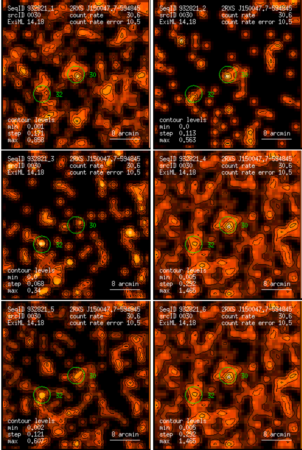
Figure 30: RASS 932821: detection 0030: band rate images, Gaussian filter: (1) PSPC channels 11 – 41, (2) 52 – 90, (3) 91 – 201, (4) 11 – 235, (5) 52 – 201, (6) 11 – 201. Broad band rates in counts/ks. Band rate contour levels in counts/ks/arcmin 2 .
