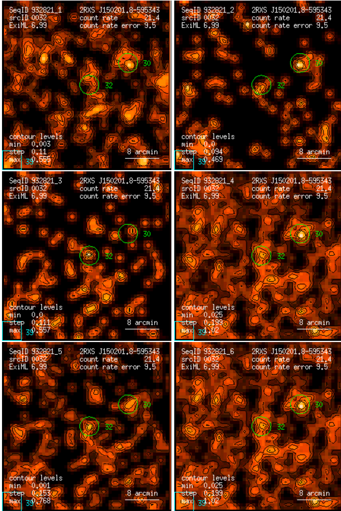
Figure 32: RASS 932821: detection 0032: band rate images, Gaussian filter: (1) PSPC channels 11 – 41, (2) 52 – 90, (3) 91 – 201, (4) 11 – 235, (5) 52 – 201, (6) 11 – 201. Broad band rates in counts/ks. Band rate contour levels in counts/ks/arcmin 2 .
