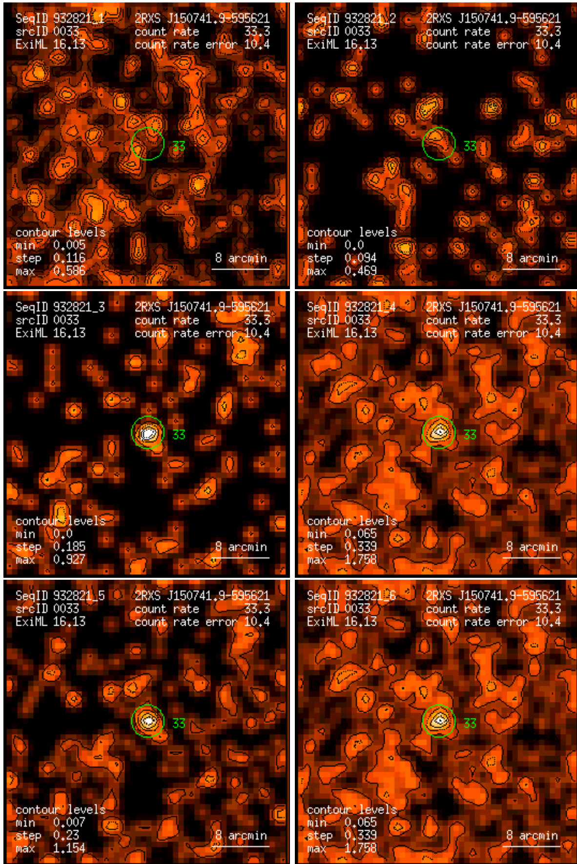
Figure 33: RASS 932821: detection 0033: band rate images, Gaussian filter: (1) PSPC channels 11 – 41, (2) 52 – 90, (3) 91 – 201, (4) 11 – 235, (5) 52 – 201, (6) 11 – 201. Broad band rates in counts/ks. Band rate contour levels in counts/ks/arcmin 2 .
