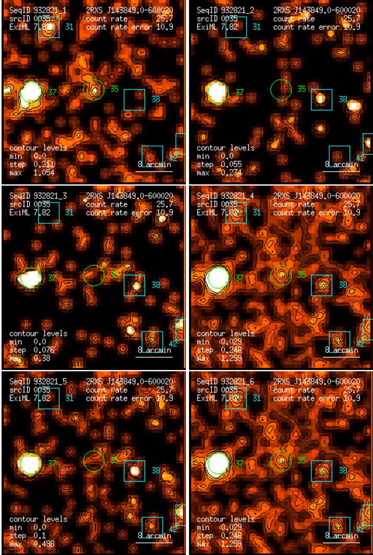
Figure 35: RASS 932821: detection 0035: band rate images, Gaussian filter: (1) PSPC channels 11 – 41, (2) 52 – 90, (3) 91 – 201, (4) 11 – 235, (5) 52 – 201, (6) 11 – 201. Broad band rates in counts/ks. Band rate contour levels in counts/ks/arcmin 2 .
