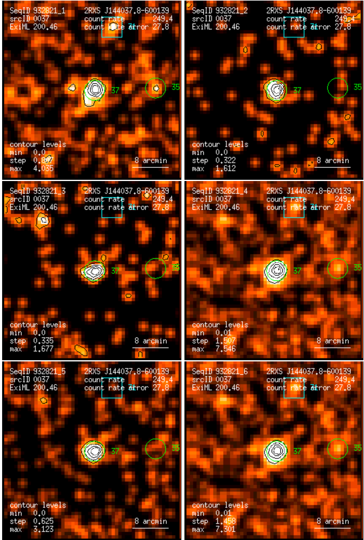
Figure 37: RASS 932821: detection 0037: band rate images, Gaussian filter: (1) PSPC channels 11 – 41, (2) 52 – 90, (3) 91 – 201, (4) 11 – 235, (5) 52 – 201, (6) 11 – 201. Broad band rates in counts/ks. Band rate contour levels in counts/ks/arcmin 2 .
