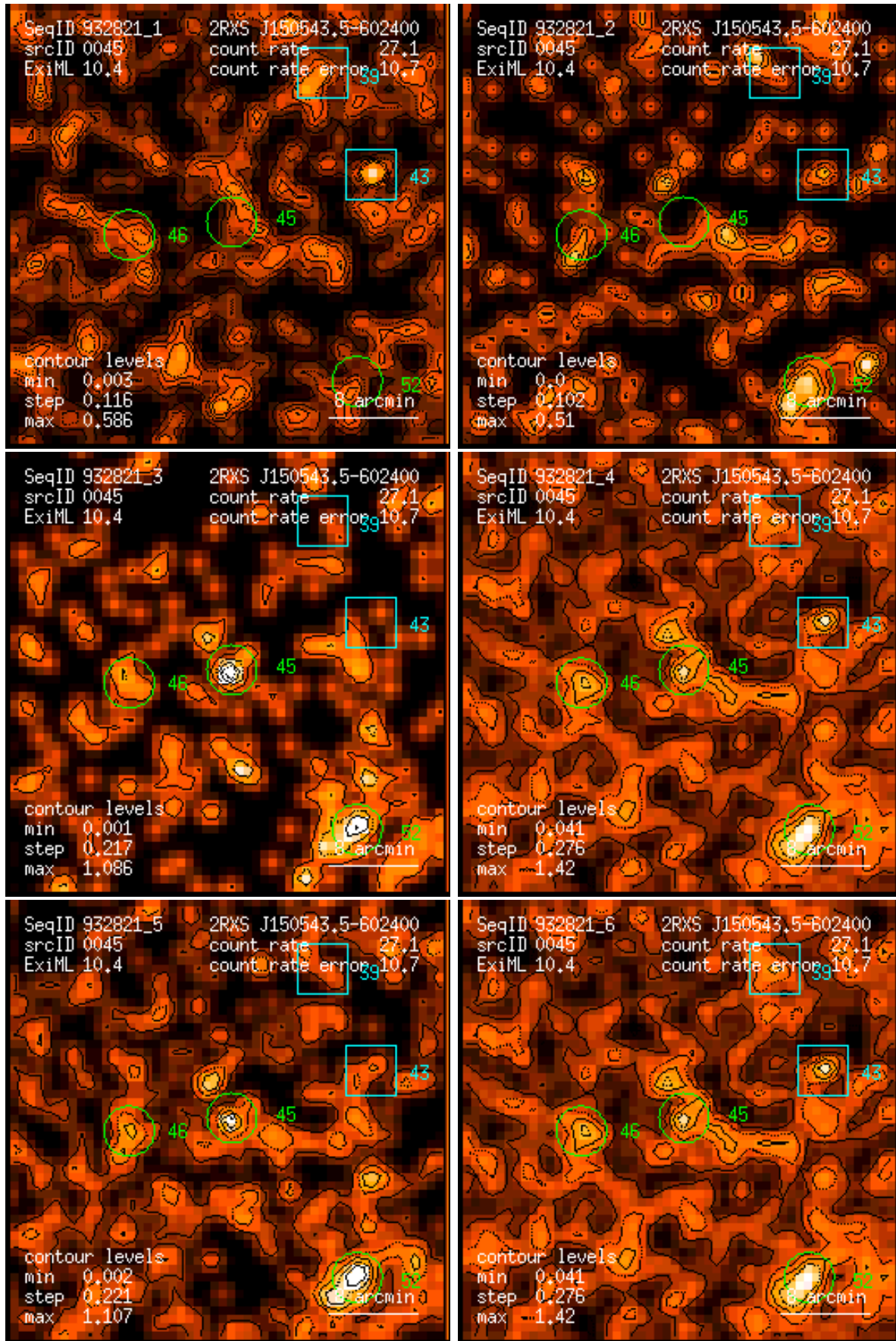
Figure 45: RASS 932821: detection 0045: band rate images, Gaussian filter: (1) PSPC channels 11 – 41, (2) 52 – 90, (3) 91 – 201, (4) 11 – 235, (5) 52 – 201, (6) 11 – 201. Broad band rates in counts/ks. Band rate contour levels in counts/ks/arcmin 2 .
