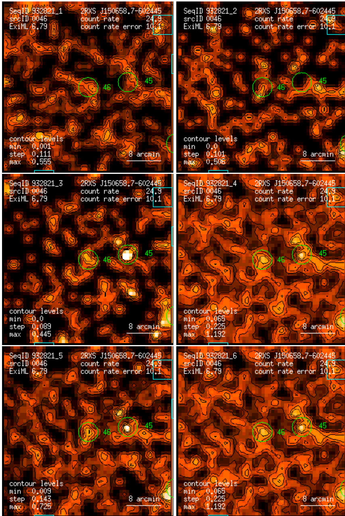
Figure 46: RASS 932821: detection 0046: band rate images, Gaussian filter: (1) PSPC channels 11 – 41, (2) 52 – 90, (3) 91 – 201, (4) 11 – 235, (5) 52 – 201, (6) 11 – 201. Broad band rates in counts/ks. Band rate contour levels in counts/ks/arcmin 2 .
