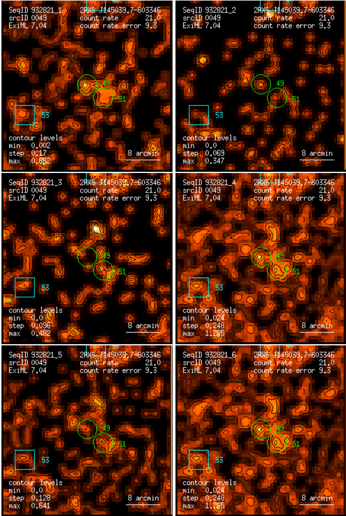
Figure 49: RASS 932821: detection 0049: band rate images, Gaussian filter: (1) PSPC channels 11 – 41, (2) 52 – 90, (3) 91 – 201, (4) 11 – 235, (5) 52 – 201, (6) 11 – 201. Broad band rates in counts/ks. Band rate contour levels in counts/ks/arcmin 2 .
