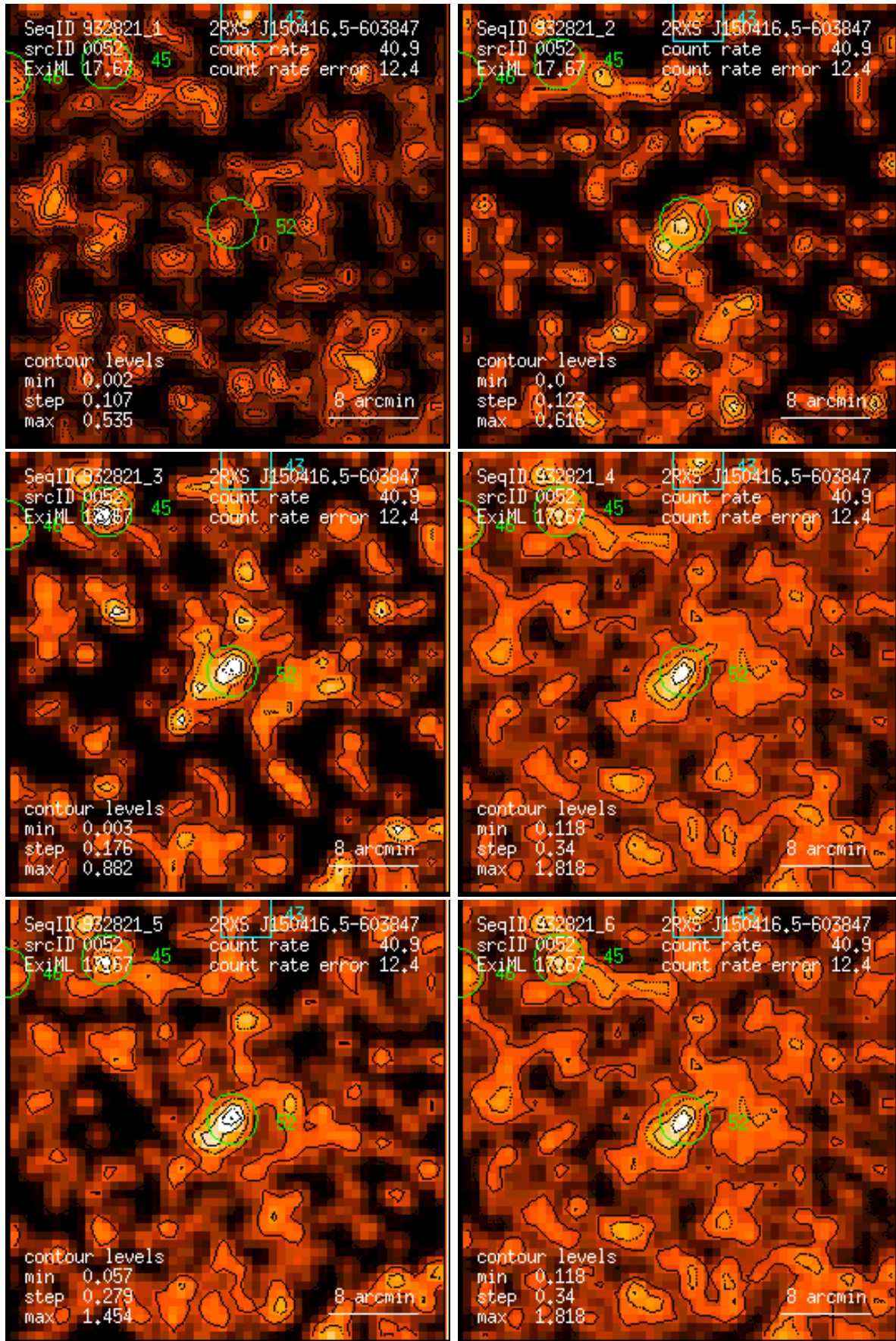
Figure 52: RASS 932821: detection 0052: band rate images, Gaussian filter: (1) PSPC channels 11 – 41, (2) 52 – 90, (3) 91 – 201, (4) 11 – 235, (5) 52 – 201, (6) 11 – 201. Broad band rates in counts/ks. Band rate contour levels in counts/ks/arcmin 2 .
