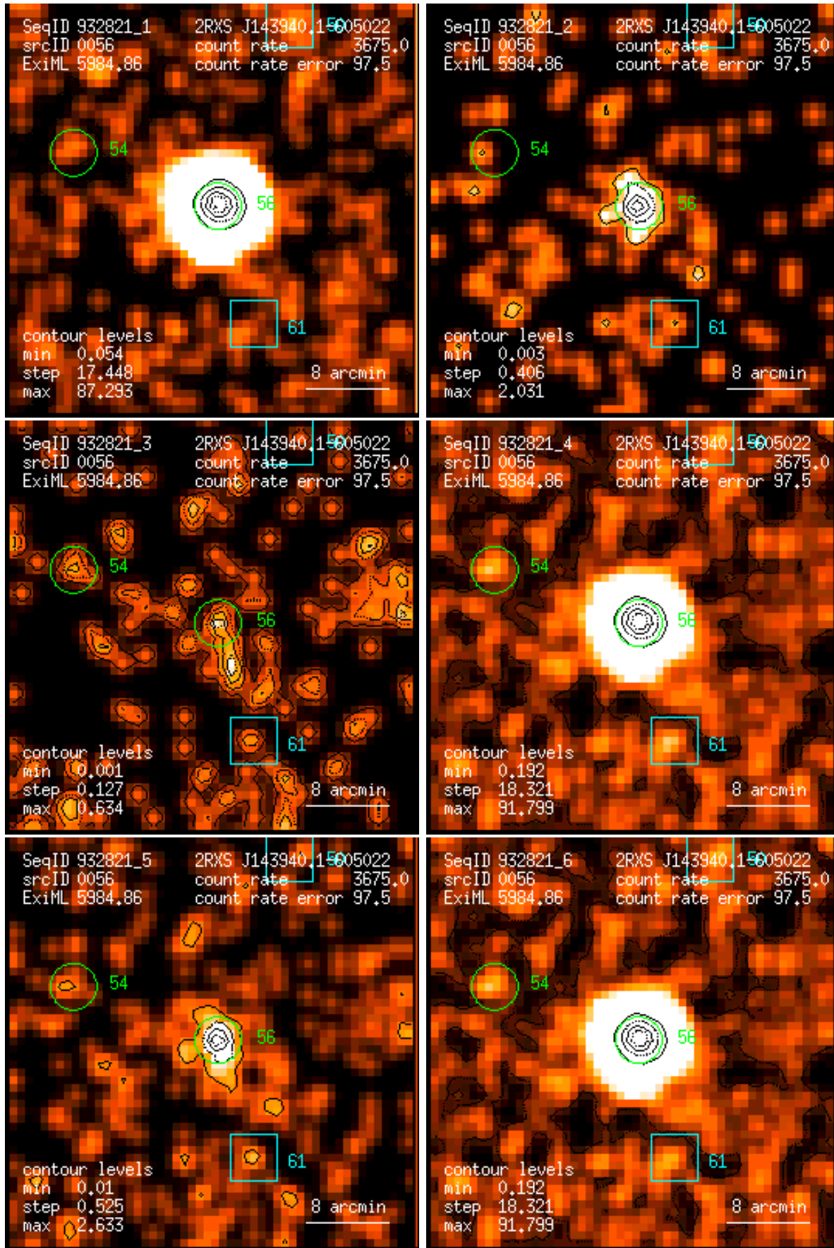
Figure 56: RASS 932821: detection 0056: band rate images, Gaussian filter: (1) PSPC channels 11 – 41, (2) 52 – 90, (3) 91 – 201, (4) 11 – 235, (5) 52 – 201, (6) 11 – 201. Broad band rates in counts/ks. Band rate contour levels in counts/ks/arcmin 2 .
