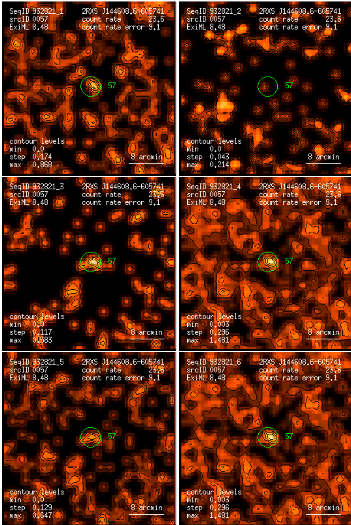
Figure 57: RASS 932821: detection 0057: band rate images, Gaussian filter: (1) PSPC channels 11 – 41, (2) 52 – 90, (3) 91 – 201, (4) 11 – 235, (5) 52 – 201, (6) 11 – 201. Broad band rates in counts/ks. Band rate contour levels in counts/ks/arcmin 2 .
