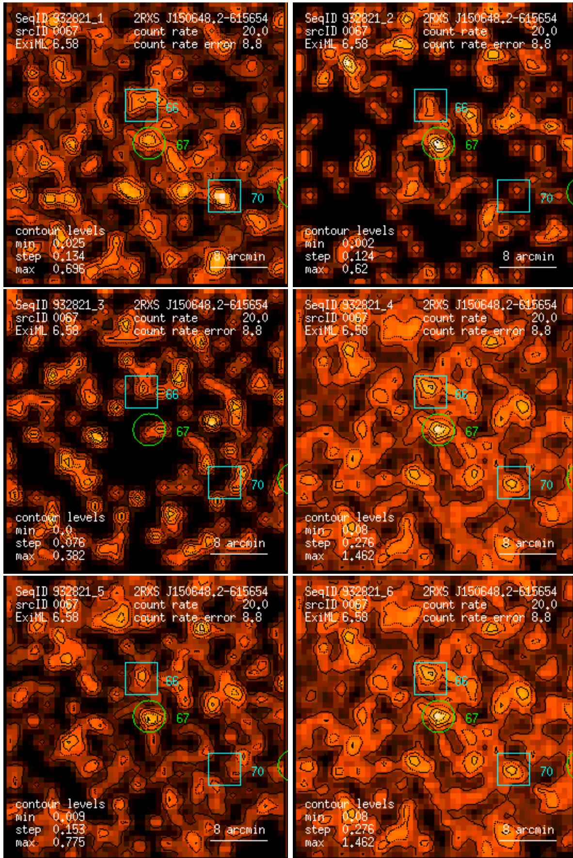
Figure 67: RASS 932821: detection 0067: band rate images, Gaussian filter: (1) PSPC channels 11 – 41, (2) 52 – 90, (3) 91 – 201, (4) 11 – 235, (5) 52 – 201, (6) 11 – 201. Broad band rates in counts/ks. Band rate contour levels in counts/ks/arcmin 2 .
