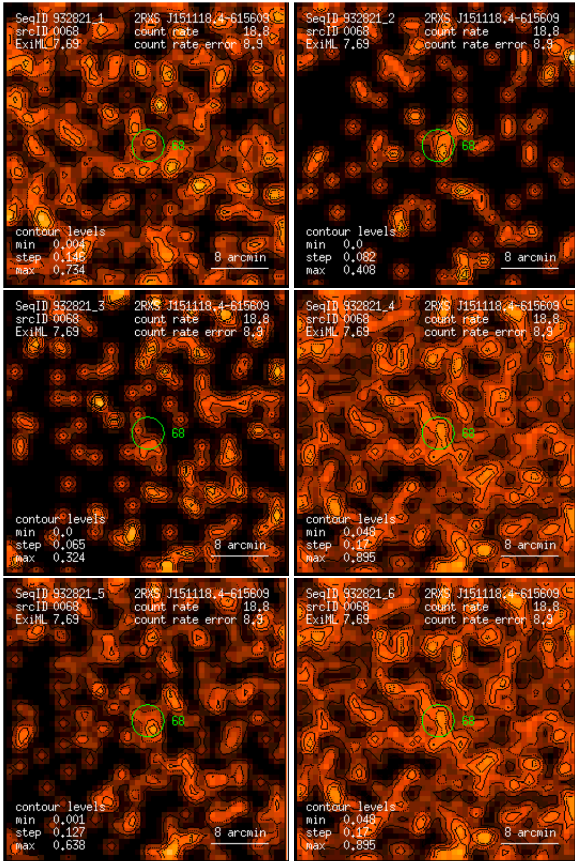
Figure 68: RASS 932821: detection 0068: band rate images, Gaussian filter: (1) PSPC channels 11 – 41, (2) 52 – 90, (3) 91 – 201, (4) 11 – 235, (5) 52 – 201, (6) 11 – 201. Broad band rates in counts/ks. Band rate contour levels in counts/ks/arcmin 2 .
