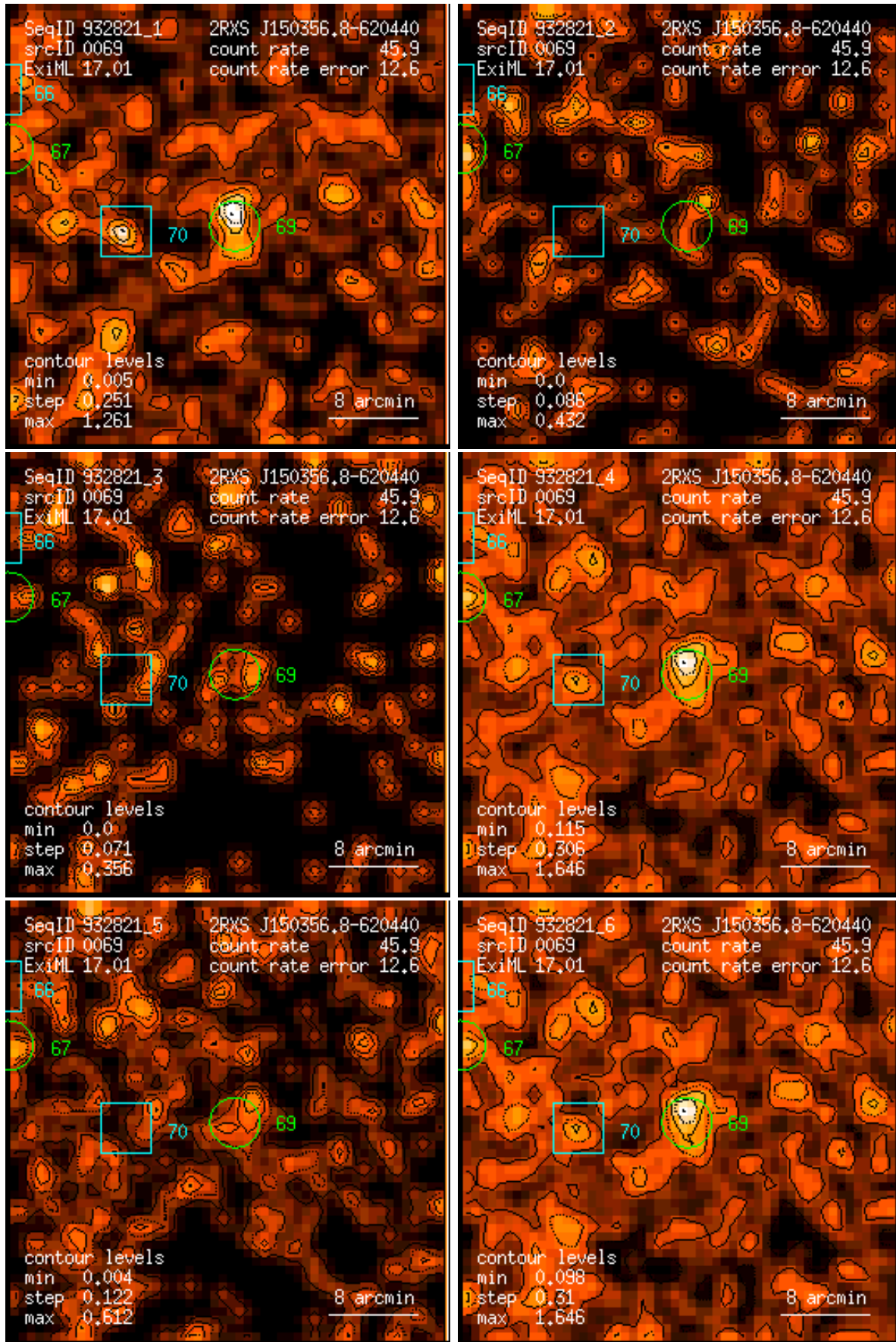
Figure 69: RASS 932821: detection 0069: band rate images, Gaussian filter: (1) PSPC channels 11 – 41, (2) 52 – 90, (3) 91 – 201, (4) 11 – 235, (5) 52 – 201, (6) 11 – 201. Broad band rates in counts/ks. Band rate contour levels in counts/ks/arcmin 2 .
