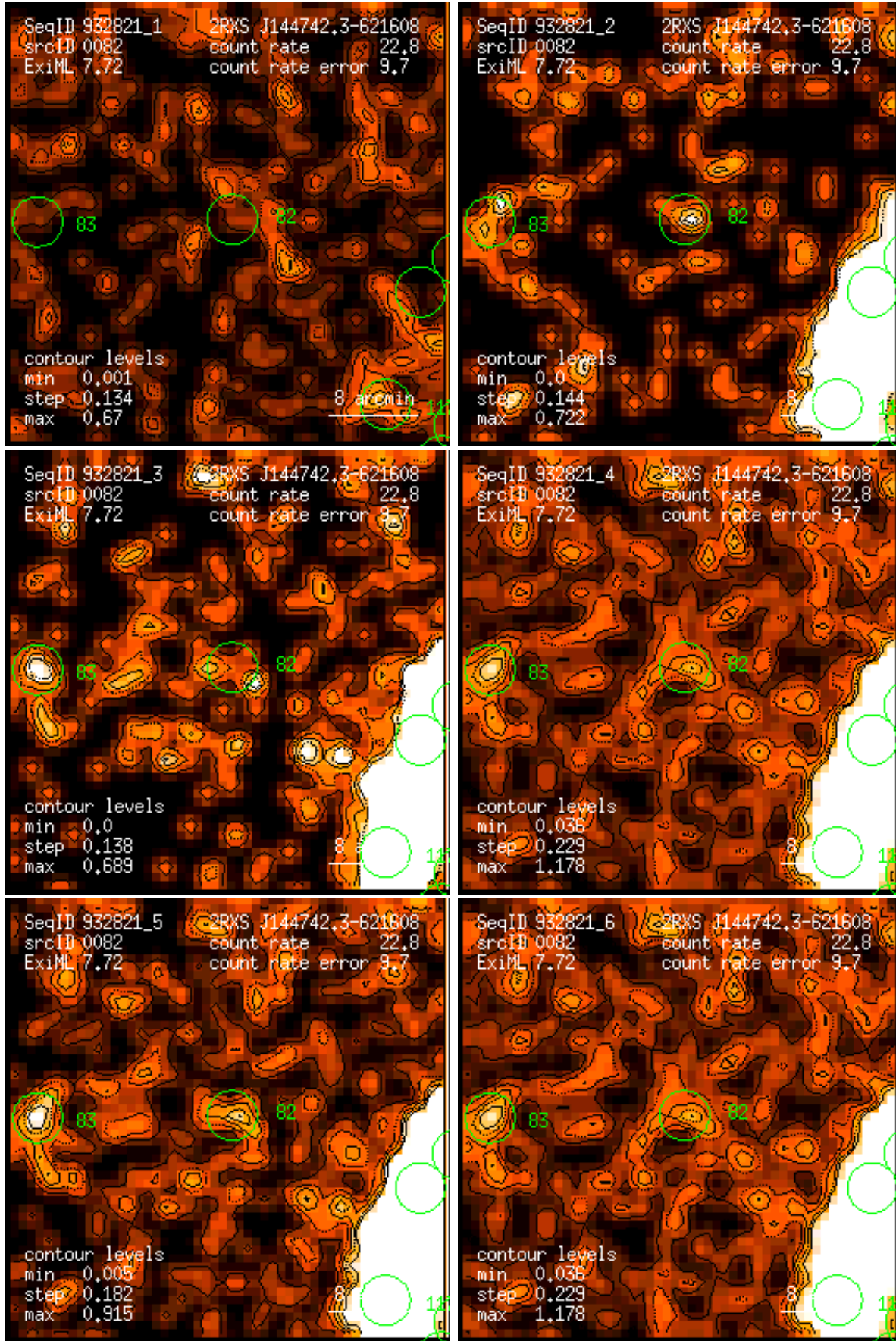
Figure 82: RASS 932821: detection 0082: band rate images, Gaussian filter: (1) PSPC channels 11 – 41, (2) 52 – 90, (3) 91 – 201, (4) 11 – 235, (5) 52 – 201, (6) 11 – 201. Broad band rates in counts/ks. Band rate contour levels in counts/ks/arcmin 2 .
