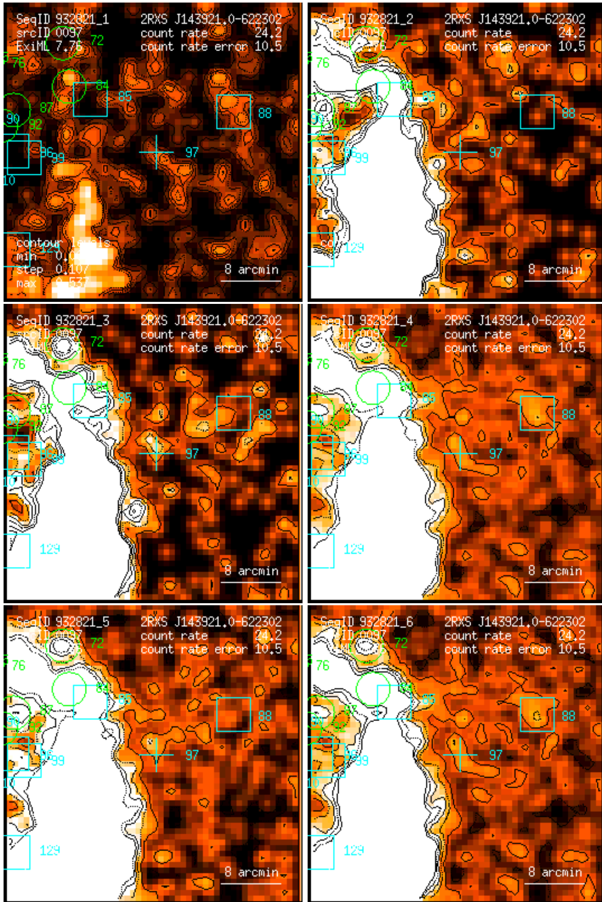
Figure 97: RASS 932821: detection 0097: band rate images, Gaussian filter: (1) PSPC channels 11 – 41, (2) 52 – 90, (3) 91 – 201, (4) 11 – 235, (5) 52 – 201, (6) 11 – 201. Broad band rates in counts/ks. Band rate contour levels in counts/ks/arcmin 2 .
